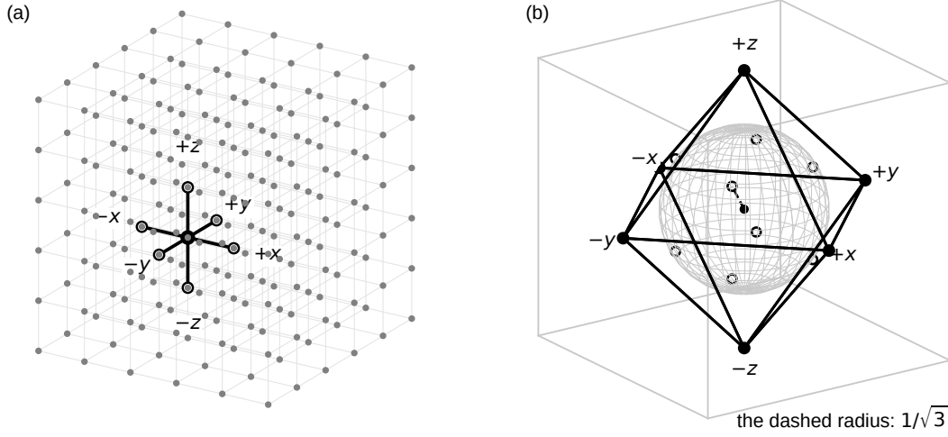
Fig. 2 (a) The GameBoard in space: a cubic array of Nodes, here 6 \times 6 \times 6 , each joined to its six neighbours by Links through the Ports \pm x , \pm y , \pm z (the faint lines). One Node and its six neighbours are marked; these are the Nodes one interval away from it. A Node keeps each family's two levels and its remainders, and nothing else. (b) The Nodes one interval away from a Node form the octahedron |x| + |y| + |z| \leq 1 , whose six vertices are the six Ports. Its symmetry group is the cube's, O_h : the 24 rotations and, with the reflections, the 48 signed permutations of the axes. Rule3 is covariant under this group (Section 3.1). The inscribed sphere, of radius 1/\sqrt{3} , touches the eight faces on the diagonals of the cube, and that radius is light's speed in Links per interval (Section 3.3). Both are drawn from the definitions; no run.
