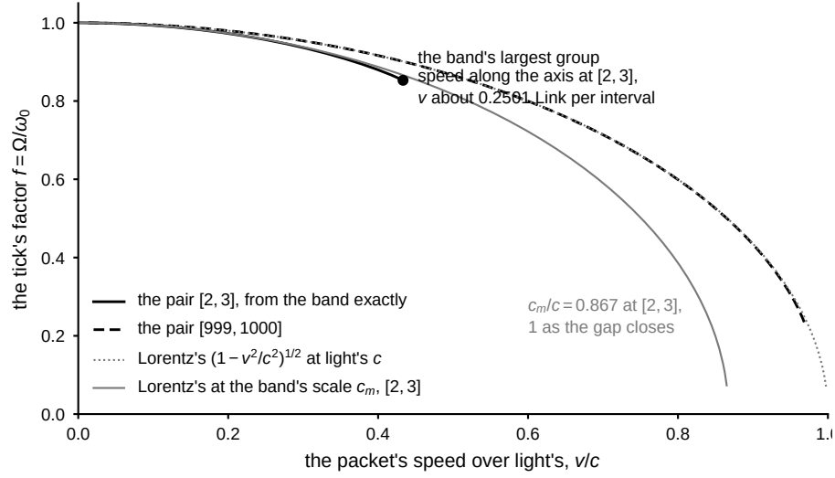
Fig. 5 The moving clock's factor from the band (Section 8, (e); DERIVED, CLICKS; drawn from the formula, no run; moving_clock.py ). A packet of a matter family moving at the velocity v = \omega'(k) along one axis ticks at the rotation at its moving centre, \Omega(k) = \omega(k) - k\omega'(k) , so its tick's factor is f = \Omega/\omega_0 . It is drawn exactly from the band for the pair [2, 3] (solid), up to the band's largest group speed along the axis, about 0.2501 Link per interval (the dot), and for the pair [999, 1000] (dashed). Beside them are Lorentz's \sqrt{1 - v^2/c^2} at light's c = 1/\sqrt{3} (dotted) and at the band's own kinetic scale c_m , c_m^2 = \omega_0/(3 \tan \omega_0) , c_m/c = 0.867 at [2, 3] (grey). The computed pair's clock follows Lorentz's at c_m to the second order, and the small-gap pair's clock follows Lorentz's at c . The factor is a property of the clicks; no boost is a symmetry of the lattice.
