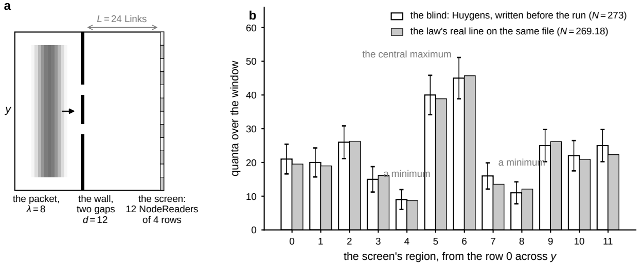
Fig. 6 The two slits, the one computed file (Sections 9.1 and 9.2; COMPUTED , CLICKS ; two.slits.rows.py ). (a) Universe24 as its file declares it. The flat GameBoard has 45 \times 48 Nodes. The packet of light, at the wavelength 8 Links, is laid over the columns 4 to 16 (the grey raised cosine) and moves along +x . The wall at the column 20 has two gaps of three rows, 12 Links apart. The screen at the column 44, 24 Links from the wall, is twelve declared NodeReaders of four rows each. (b) The screen's row per region over the window of the intervals 45 to 130. The Huygens blind, written before the run, is hollow ( N = 273 , with the draw's scatter \sqrt{Np(1-p)} per region). Beside it, in grey, is the law's real line stepped on the same file, as printed in two.slits.real.line.txt by the paper's script two.slits.real.line.py at the lay as the pinned commit holds it ( N = 269.18 in the engine's labels, 269.3 in the physical ones). The run of the implementation gives N = 270 (Section 3.7). The numbers drawn are the blind file's and the script's; nothing is read from a run of the engine for the drawing.
