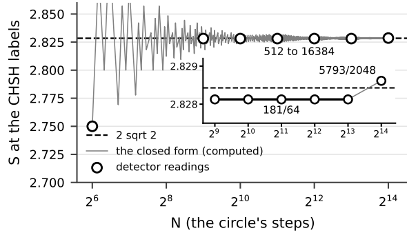
Figure 4: S(N_\phi) at the CHSH labels. The curve is the closed form S(N_\phi) = 8(c_1 + c'_1)/N_\phi - 4 computed from the rule at every multiple of 8 with the tables at N_t = 256 , a computation [5]; the circles are detector readings (DETECTOR) at N_\phi = 64, 512, 1024, 2048, 4096, 8192 and 16384 (series L, L6 and the register's block of the derivation's 24.4, the last three [4, at b34fe114]); the inset marks the plateau 181/64 from 512 through 8192 and its end 5793/2048 at 16384 ; the dashed line is 2\sqrt{2} .
