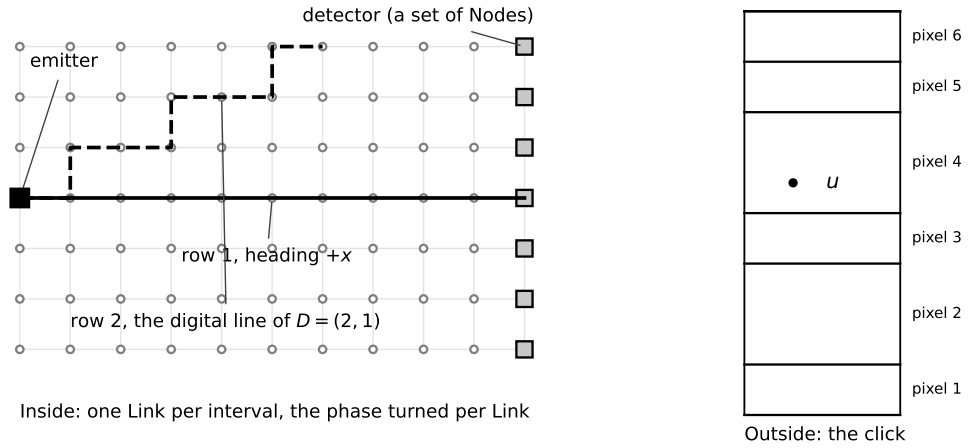
Figure 1: The mechanism, drawn from the definitions and no run. Inside (left): a GameBoard of Nodes joined by Links; an emitter puts one record of two rows on the board, each row on the digital line of its direction at one Link per interval, its phase turned per Link, nothing kept at a Node; a detector is a set of Nodes. Outside (right): the click, one comparison of the record's birth phase u against the rungs of its ladder (Eq. (9)); the cell u falls in is the outcome, and the record is deleted. Nothing else is read.
