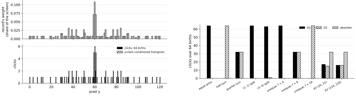
Figure 2: Interference read at a detector, from the runs of series L at N_\phi = 64 (the figures' runs, Appendix C). Left, the two-slit world slits_huygens : above, the record's weight per pixel of the screen, a number of the board (GAMEBOARD, a diagnostic); below, the clicks over 64 births (DETECTOR) and the histogram conditioned on the screen, bright where the two rows' ages differ by whole turns. Right, the Mach-Zehnder worlds: the clicks over 64 births at the two ports and the absorber (DETECTOR), equal arms 64/0, a half turn 0/64, a quarter turn 32/32, the (1,1) and (3,4) splits, the unequal arms and the two Elitzur-Vaidman worlds (Table 2, row 2b; Appendix C).
