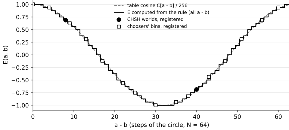
Figure 3: The pair at N_\phi = 64 : E(a, b) computed from the rule at every setting difference a - b (the counts of Theorem 5 with the repository's tables, a computation [5]), the tables' cosine C[a - b]/256 dashed, and after a detector the registered CHSH worlds (circles) and the choosers' bins (squares) of series L (DETECTOR).
