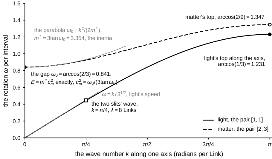
Fig. 3 Light's and matter's bands along one axis, from the law's line (DERIVED, GAMEBOARD; drawn from the formula, no run): \cos \omega = \frac{\text{num}}{3 \text{ den}} (2 + \cos k) at the wave number k along one axis, light's pair [1, 1] (solid) and matter's [2, 3] (dashed). At k = 0 the gap \cos \omega_0 = \text{num}/\text{den} , 0.841 for matter, with the parabola \omega_0 + k^2/(2m^*) of the inertia m^* = 3 \tan \omega_0 = 3.354 (grey); at k = \pi the band's top \arccos(\text{num}/(3 \text{ den})) , 1.231 for light and 1.347 for matter; light's slope at the origin is its speed 1/\sqrt{3} Links per interval (grey), and the two slits' wave, k = \pi/4 (the square), sits on light's band at \omega = 0.4456 , the period 14.1 intervals (Section 9.1). E = m^* c_m^2 = \omega_0 exactly, with c_m^2 = \omega_0/(3 \tan \omega_0) ; along the cube's diagonal light has \cos \omega = \cos k , no dispersion, not drawn.
