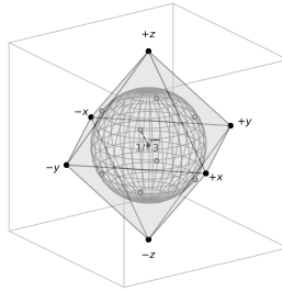
Figure 1: The Nodes one interval from a Node: the six neighbours are the vertices of the octahedron |x| + |y| + |z| \leq 1 , the causal front of one interval; its inscribed sphere, of radius 1/\sqrt{3} , touches the eight faces on the cube diagonals and is the rows' pace c (Proposition 1); the faint cube shares the 48 signed permutations of the axes. Drawn by octahedron.py from the definitions; no run.
