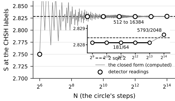
Figure 2: S(N_\phi) at the CHSH labels. The curve is the closed form S(N_\phi) = 8(c_1 + c'_1)/N_\phi - 4 computed from the rule at every multiple of 8 with the tables at N_t = 256 , a computation [5]; the circles are detector readings (DETECTOR) at N_\phi = 64, 512, 1024, 2048, 4096, 8192 and 16384 (series L, L6 and the register's block of the derivation's 24.4, the last three on main at b34fe114 ); the inset marks the plateau 181/64 from 512 through 8192 and its end 5793/2048 at 16384 ; the dashed line is 2\sqrt{2} .
