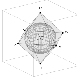
Figure 1: The Nodes one interval from a Node: the six neighbours are the vertices of the octahedron |x| + |y| + |z| \leq 1 , the causal front of one interval; its inscribed sphere, of radius 1/\sqrt{3} , touches the eight faces on the cube diagonals and is the rows' pace c (Proposition 1); the faint cube shares the 48 signed permutations of the axes. Drawn by octahedron.py from the definitions; no run.
