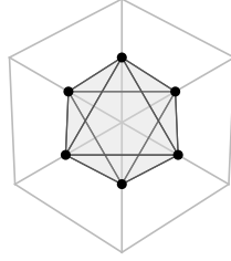
Figure 1: From the groups to the click. Left: the six Ports as the face centres of a cube, the symmetry group of the cube (48, its rotations the group of order 24), and the octahedron they span, the causal front of one interval. Second: the same six Ports along a body diagonal, a hexagon, the cubic pattern of the dispersion. Third: the GameBoard with the block inside it, the block itself the detector, its cells the detector set with the rung W ; the phase circle \mathbb{Z}_{N_\phi} on it, the record's clock, tied to the record's pair by the kind's declared clock (light's phase per Link [n, d] , the massive kind's \cos \omega_0 = \text{num}/\text{den} ); the light record running on the free Nodes and through the block; the take a declaration of the world file. Right: the click, the quadratic form of the record's values in the cells crossing the rung, one per record, the only thing that leaves the board; every other number of the paper is a GAMEBOARD reading of the host. Drawn from the definitions by groups.figure.py ; no run.
