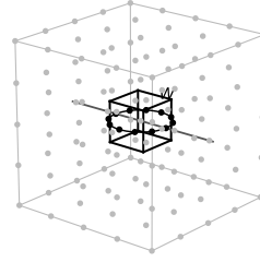
Figure 1: From the groups to the click. Left: the six Ports as the face centres of a cube, the symmetry group of the cube (48, its rotations the group of order 24), and the octahedron they span, the causal front of one interval. Second: the same six Ports along a body diagonal, a hexagon, the cubic pattern of the dispersion. Third: the GameBoard with the block inside it, the block itself the detector, its cells the detector set with the rung W ; the phase circle \mathbb{Z}_{N_\phi} on it, the record's clock, tied to the record's pair by the kind's declared clock (light's phase per Link [n, d] , the massive kind's \cos \omega_0 = \text{num}/\text{den} ); the light record running on the free Nodes and through the block; the take a declaration of the world file. Right: the click, the quadratic form of the record's values in the cells crossing the rung, one per record, the only thing that leaves the board; every other number of the paper is a GAMEBOARD reading of the host. Drawn from the definitions by groups.figure.py ; no run.
