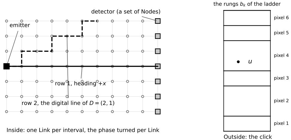
Figure 2: The mechanism, drawn from the definitions and no run. Inside (left): a GameBoard of Nodes joined by Links; an emitter puts one record of two rows on the board, each row on the digital line of its direction at one Link per interval, its phase turned per Link, nothing kept at a Node; a detector is a set of Nodes. Outside (right): the click, one comparison of the record's birth phase u against the rungs of its ladder (Eq. (9)); the cell u falls in is the outcome, and the record is deleted. Nothing else is read.
