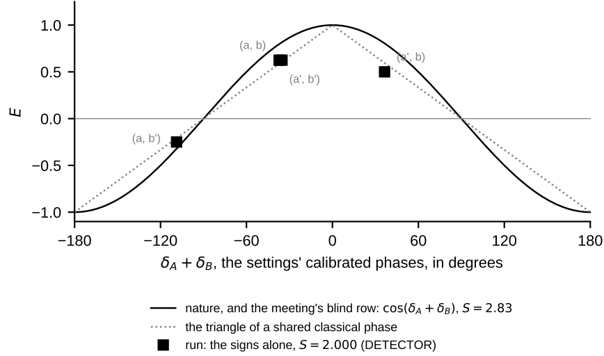
Fig. 8 Bell: the correlation E at the four settings against the sum of the settings' calibrated phases. The run by the signs alone on both sides, every quantum credited (the marks, DETECTOR), follows the triangle of a shared classical phase and sums to S = 2.000 ; the cosine is nature's E = \cos(\delta_A + \delta_B) and the meeting's blind row, S = 2.83 , for the run to come. Drawn from the rows of the law's document; no run of this paper's.
