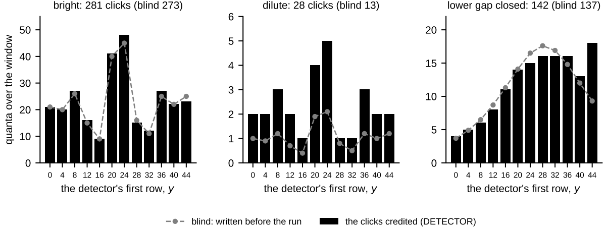
Fig. 7 The two slits: the clicks credited to each of the screen's twelve declared detectors (the bars, DETECTOR, the measurement) beside the blind row written before the run (the dashed line), for the bright packet, the dilute packet and the world with the lower gap closed; each detector a region of four rows named by its first row. The fringes stand at the near field's places, the minima at the rows 15 and 33 and the outer maxima in the edge regions; with one gap closed the screen gives one gap's envelope and no fringes. Drawn from the rows of the law's document; no run of this paper's.
