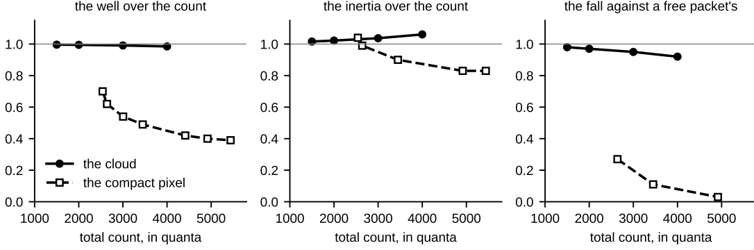
Fig. 6 The three masses of a body along its two branches, from the documents' rows (DERIVED from the fixed point, a reading of the algebra and no click; the counts in the advisor's unit): the well over the count, the inertia over the count and the fall against a free packet's, for the cloud (the wide branch, filled marks) against its total count, and for the compact pixel (the narrow branch, open marks) against its total count. For the cloud the three go to one and the fall to a free quantum's the wider it is; for the compact pixel they part by the binding. Drawn from the rows of the law's document; no run.
