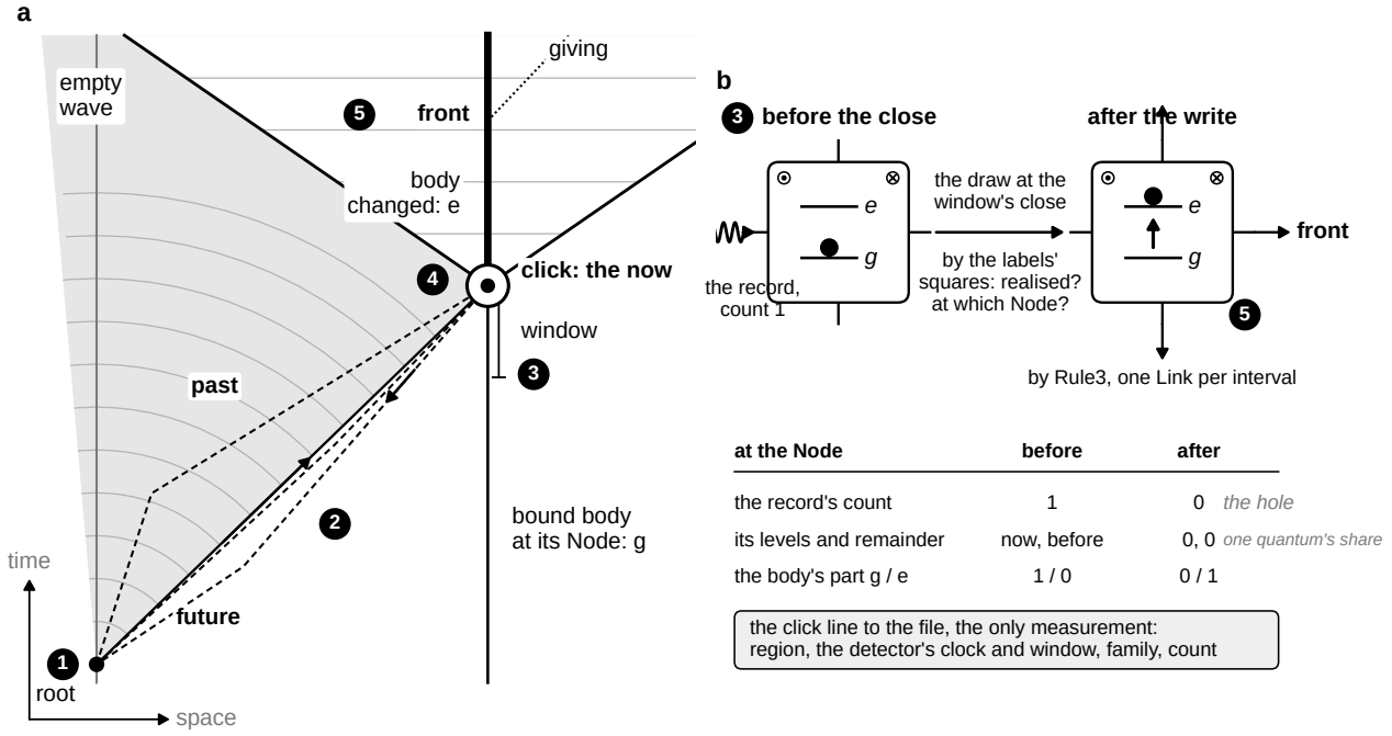
Fig. 4 The click at a bound body, schematically (ASSUMPTION; drawn from the definitions, no run; black and grey, solid lines run forward and dashed lines read backward). (a) Space and time at the body's one Node. 1: the giver's record is laid at its root and runs forward by Rule3, every path at once (the grey fan with its wavefronts, the future). 2: the bound body stands at its Node with its part g laid. The window (3, the bracket) opens at the body's last write and closes at the probe's taking. At the close the arriving quantum meets the body's own transition, and the instrument draws with its declared seed: the click, the now (the ring). 4: from the click the same line is read backward, Rule3 at -1 , through every path (the dashed lines, the past); this is a reading and never a write. 5: forward, the body is changed: its part e is laid and the quantum is held until its giving (the thick line; the dotted line is the giving when it comes). The change spreads by Rule3 at one Link per interval, the front (the white cone), and erases the record that gave inside the click's light cone. Beyond the front the record's levels remain, the empty wave with count 0, stepped on and never credited. (b) The one Node, its six Ports (four in the plane, two out of it), and the body's parts g and e as a ladder with the laid part filled, before the window's close and after the one write. At the close, the share D = \text{now}^2 - \text{next} \times \text{before} at the Node. The window's turn sets the labels, and the draw with the seed is by their squares: whether it is realised, and at which one Node. After it, the hole: the record's levels and remainder at that Node go to 0 for one quantum's share, scaled where the record is denser; its count goes down by one, g down by one and e laid up by one; Rule3 steps the change on through the Ports. The click line, with the region, the detector's own clock and the window's index, the family and the count, goes to the detector's file: the report and the only measurement.
