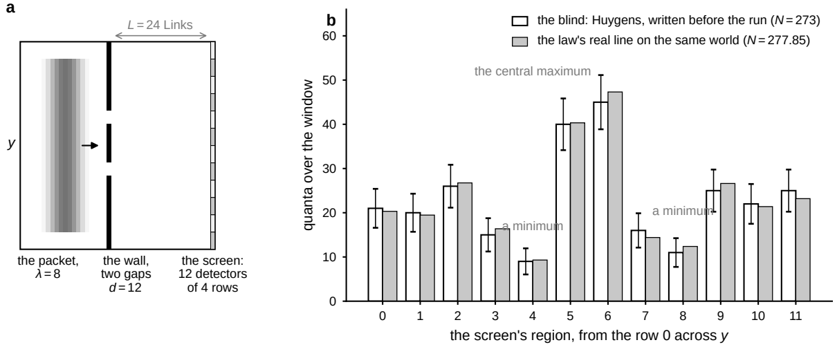
Fig. 6 The two slits, the one computed world (Sections 9.1 and 9.2; COMPUTED, CLICKS). (a) The world as its file declares it. The flat GameBoard has 45 \times 48 Nodes. The packet of light, at the wavelength 8 Links, is laid over the columns 4 to 16 (the grey raised cosine) and moves along +x . The wall at the column 20 has two gaps of three rows, 12 Links apart. The screen at the column 44, 24 Links from the wall, is twelve declared detectors of four rows each. (b) The screen's row per region over the window of the intervals 45 to 130. The Huygens blind, written before the run, is hollow ( N = 273 , with the draw's scatter \sqrt{Np(1-p)} per region). Beside it, in grey, is the law's real line stepped on the same world by the paper's script two_slits_real_line.py ( N = 277.85 in the engine's labels, 278.0 in the physical ones). The run of the implementation gives N = 278 (Section 3.7). The numbers drawn are the blind file's and the script's; nothing is read from a run of the engine for the drawing.
