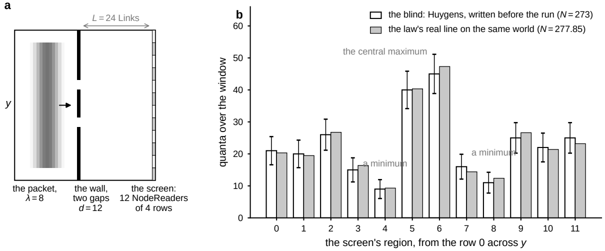
Fig. 6 The two slits, the one computed setup (Sections 9.1 and 9.2; COMPUTED, CLICKS). (a) The setup as its file declares it. The flat GameBoard has 45 \times 48 Nodes. The packet of light, at the wavelength 8 Links, is laid over the columns 4 to 16 (the grey raised cosine) and moves along +x . The wall at the column 20 has two gaps of three rows, 12 Links apart. The screen at the column 44, 24 Links from the wall, is twelve declared NodeReaders of four rows each. (b) The screen's row per region over the window of the intervals 45 to 130. The Huygens blind, written before the run, is hollow ( N = 273 , with the draw's scatter \sqrt{Np(1-p)} per region). Beside it, in grey, is the law's real line stepped on the same setup by the paper's script two_slits_real_line.py ( N = 277.85 in the engine's labels, 278.0 in the physical ones). The run of the implementation gives N = 278 (Section 3.7). The numbers drawn are the blind file's and the script's; nothing is read from a run of the engine for the drawing.
