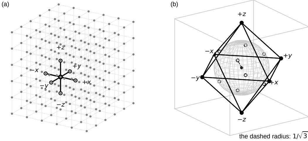
Fig. 2 (a) The GameBoard in space: a cubic array of Nodes, here 6 \times 6 \times 6 , each joined to its six neighbours by Links through the Ports \pm x, \pm y, \pm z (the faint lines). One Node and its six neighbours are marked; these are the Nodes one interval away from it. A Node keeps each family's two levels and its remainders, and nothing else. (b) The Nodes one interval away from a Node form the octahedron |x| + |y| + |z| \leq 1 , whose six vertices are the six Ports. Its symmetry group is the cube's, O_h : the 24 rotations and, with the reflections, the 48 signed permutations of the axes. Rule3 is covariant under this group (Section 3.1). The inscribed sphere, of radius 1/\sqrt{3} , touches the eight faces on the diagonals of the cube, and that radius is light's speed in Links per interval (Section 3.3). Both are drawn from the definitions; no run.
