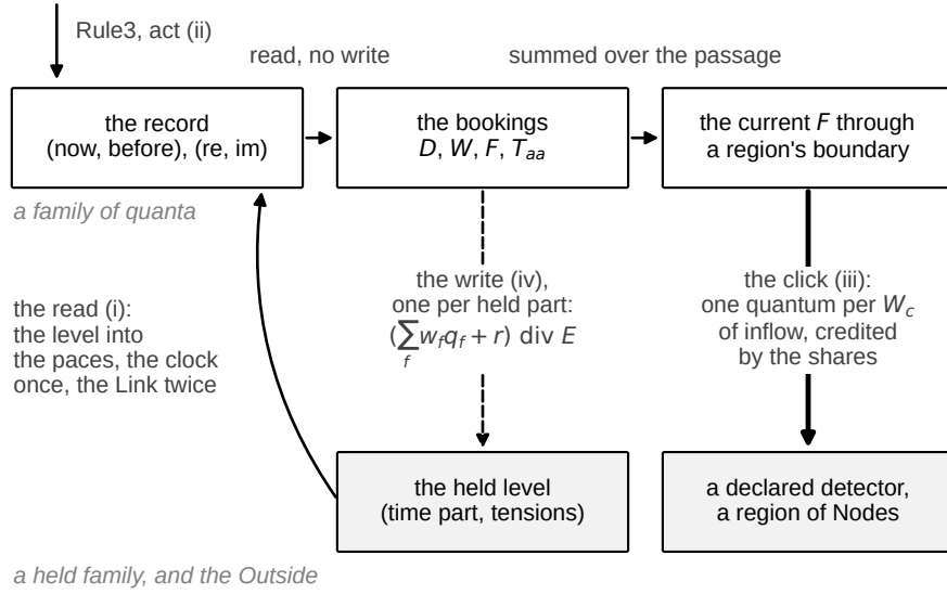
Fig. 4 The three channels through which a family acts on another, drawn from the interval's four acts (Section 2.5). A family of quanta steps its record by Rule3 and books its form and its current; a field family carries a level. The read (i) takes the field's level into the record's paces; the write (iv) takes the record's form, its Wronskian's quanta and its tension into the field's level over the field's divisor; the click (iii) is a declared region's reading of the current through its boundary, summed over the passage, one quantum per wall W_c of inflow, credited by the instrument; the write (iv) is one division per held part of the summed sources. Every arrow is one line of Eq. (1). Drawn from the definitions; no run.
