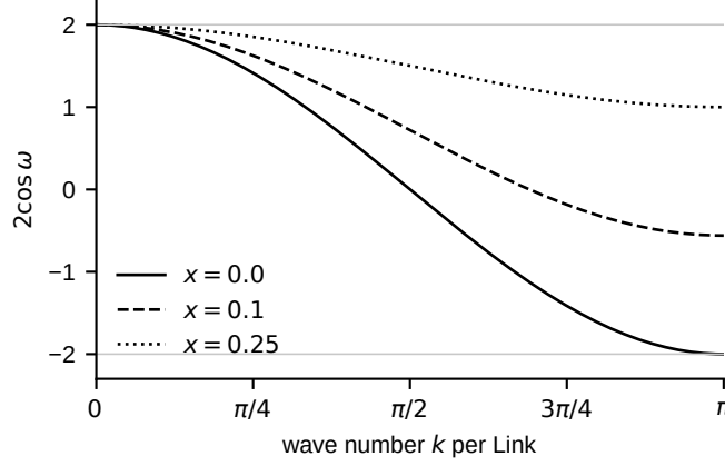
Fig. 3 Light's band at a content x = L/\Gamma read into the paces (DERIVED, Eq. (4) at num = den): the doubled cosine of the rotation along one axis against the wave number, 2 \cos \omega = 2 - 2(1 - 2x)^2(1 - \cos k) , at x = 0, 0.1 and 0.25 . The band's bottom rises with the content, its top stays at 2; at the horizon x = 1/2 the band closes to a point. The slope at k = 0 is light's speed, (1 - 2x)/\sqrt{3} Links per interval. Drawn from the definitions; no run.
