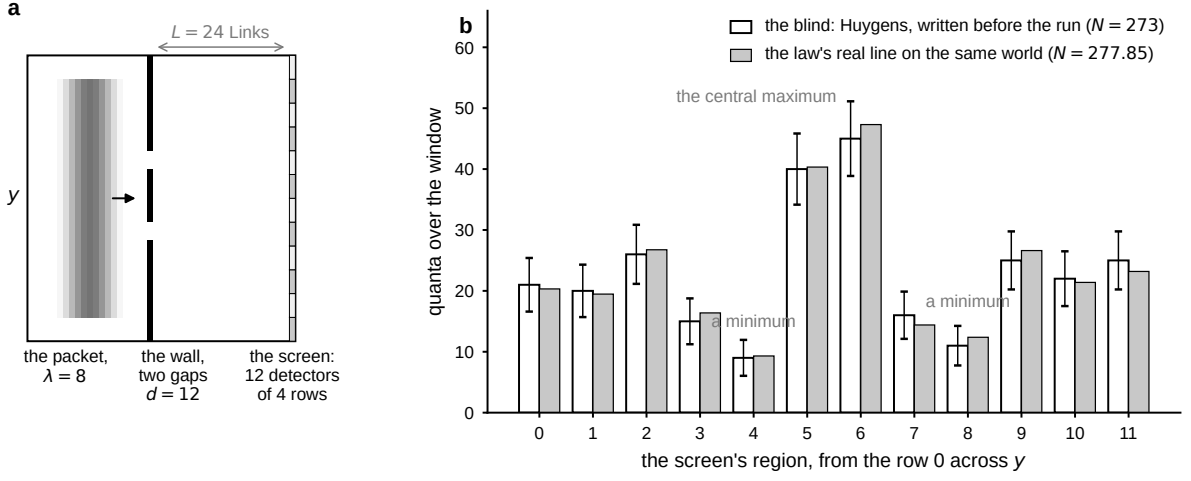
Fig. 4 The two slits, the one computed world (Sections 9.1 and 9.2; COMPUTED, CLICKS). (a) The world as its file declares it: the flat GameBoard of 45 \times 48 Nodes, the packet of light at the wavelength 8 Links laid over the columns 4 to 16 (the grey raised cosine) and moving along +x , the wall at the column 20 with two gaps of three rows 12 Links apart, the screen at the column 44, 24 Links from the wall, twelve declared detectors of four rows each. (b) The screen's row per region over the window of the intervals 45 to 130: the Huygens blind written before the run (hollow, N = 273 , with the draw's scatter \sqrt{Np(1-p)} per region) beside the law's real line stepped on the same world by the paper's script two_slits_real_line.py (grey, N = 277.85 in the engine's labels, 278.0 in the physical ones); the run of the implementation gives N = 278 (Section 3.7). The numbers drawn are the blind file's and the script's; nothing is read from a run of the engine for the drawing.
