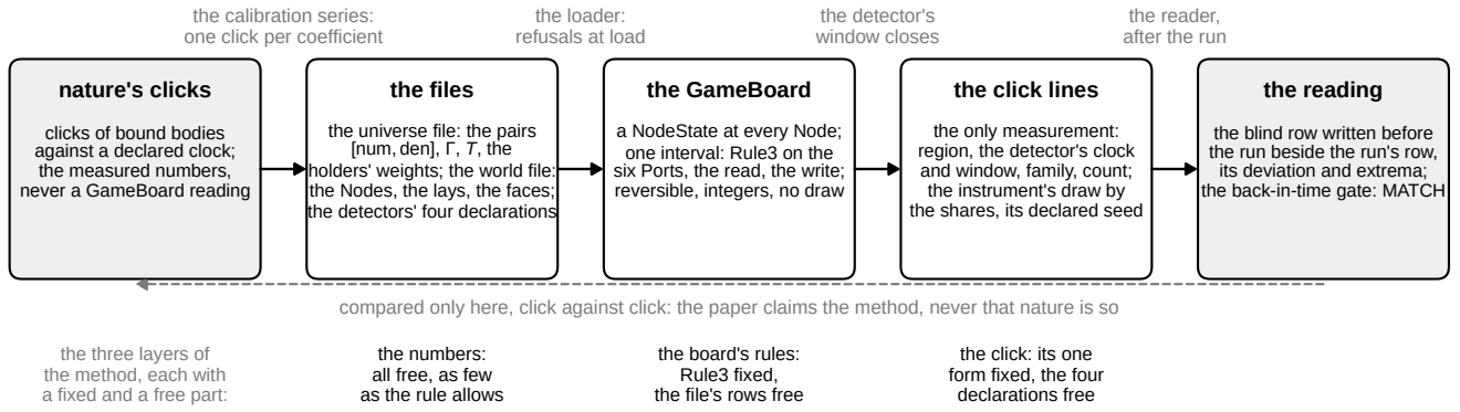
Fig. 5 The method, from nature's clicks to the paper's reading (Sections 1, 3.7, 5.3 and 10.2; drawn from the definitions, no run). Nature's clicks on bound bodies are read, one click per coefficient, into the files' integers, the calibration series; the files declare the world; the GameBoard is stepped by Rule3, one interval of acts on the six Ports, reversible, in whole numbers and with no draw; the detectors write the click lines, the only measurement; the reader prints the run's row beside the blind row written before the run, with the back-in-time gate's MATCH; and only there, click against click, the computed world meets the clicks it approaches: the paper claims the method, never that nature is so. Below the boxes, the three layers, each with its fixed and its free part.
