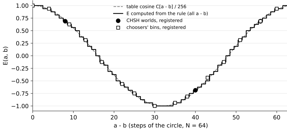
Figure 4: The pair at N_\phi = 64 : E(a, b) computed from the rule at every setting difference a - b (the counts of Theorem 5 with the repository's tables, a computation [5]), the tables' cosine C[a - b]/256 dashed, and after a detector the registered CHSH worlds (circles) and the choosers' bins (squares) of series L (DETECTOR).
