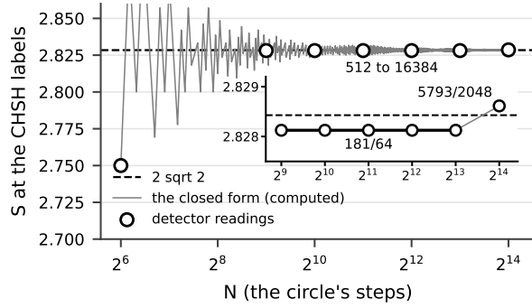
Figure 5: S(N_\phi) at the CHSH labels. The curve is the closed form S(N_\phi) = 8(c_1 + c'_1)/N_\phi - 4 computed from the rule at every multiple of 8 with the tables at N_t = 256 , a computation [5]; the circles are detector readings (DETECTOR) at N_\phi = 64, 512, 1024, 2048, 4096, 8192 and 16384 (series L, L6 and the register's block of the derivation's 24.4, the last three [4, at b34fe114]); the inset marks the plateau 181/64 from 512 through 8192 and its end 5793/2048 at 16384 ; the dashed line is 2\sqrt{2} .
