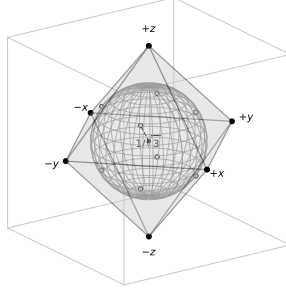
Figure 2: The Nodes one interval from a Node: the six neighbours are the vertices of the octahedron |x| + |y| + |z| \leq 1 , the causal front of one interval; its inscribed sphere, of radius 1/\sqrt{3} , touches the eight faces on the cube diagonals and is the rows' pace c (Proposition 1); the faint cube shares the 48 signed permutations of the axes. Drawn by octahedron.py from the definitions; no run.
