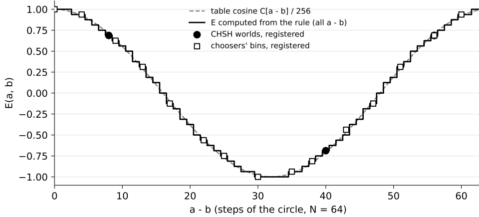
Figure 5: The pair at N_\phi = 64 : E(a, b) computed from the rule at every setting difference a - b (the counts of Theorem 5 with the repository's tables, a computation [5]), the tables' cosine C[a - b]/256 dashed, and after a detector the registered CHSH worlds (circles) and the choosers' bins (squares) of series L (DETECTOR).
