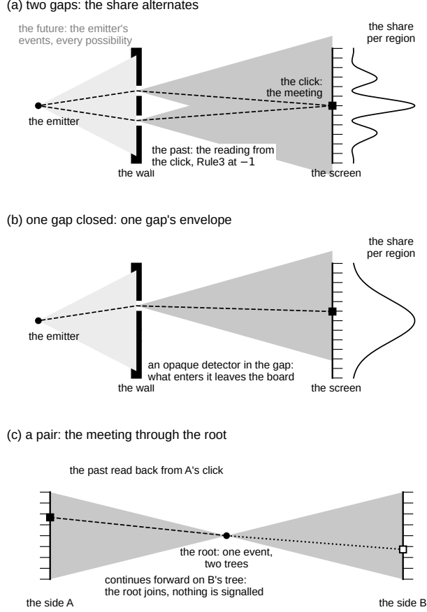
Fig. 2 The click as the meeting of the future with the past, schematically (ASSUMPTION; drawn from the definitions, no run). (a) The two slits: the emitter's events spread forward through both gaps, every possibility at once (the grey fans, the future); from a realised click at the screen the same line is read backward, Rule3 at -1 , through both gaps (the dashed lines, the past); the share along the screen, the product of the two directions, alternates. (b) One gap closed by an opaque detector: the backward reading meets one gap and the share is one gap's envelope. (c) A pair, two trees with one root: the backward reading from A's click passes the root and continues on B's tree (the dotted line); nothing is signalled.
