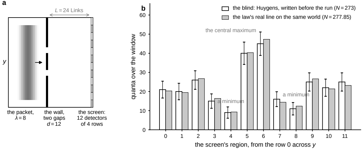
Fig. 5 The two slits, the one computed world (Sections 9.1 and 9.2; COMPUTED, CLICKS). (a) The world as its file declares it: the flat GameBoard of 45 \times 48 Nodes, the packet of light at the wavelength 8 Links laid over the columns 4 to 16 (the grey raised cosine) and moving along +x , the wall at the column 20 with two gaps of three rows 12 Links apart, the screen at the column 44, 24 Links from the wall, twelve declared detectors of four rows each. (b) The screen's row per region over the window of the intervals 45 to 130: the Huygens blind written before the run (hollow, N = 273 , with the draw's scatter \sqrt{Np(1-p)} per region) beside the law's real line stepped on the same world by the paper's script two.slits.real.line.py (grey, N = 277.85 in the engine's labels, 278.0 in the physical ones); the run of the implementation gives N = 278 (Section 3.7). The numbers drawn are the blind file's and the script's; nothing is read from a run of the engine for the drawing.
