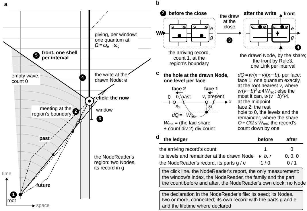
Fig. 4 The click at a NodeReader, in plain words (ASSUMPTION for the draw and the write, the rest DERIVED; CLICKS; drawn from the definitions, no run; solid lines run forward, dashed lines read backward). A NodeReader is where the future meets the past: the arriving record's quantum, run forward from its root, is the future; the quantum of the transition that waits for it, read back from the realised click, is the past; the click is their meeting, the present, and there is no click of one quantum alone. (a) Space and time. 1: the arriving record runs forward from its root by Rule3, every path at once (the grey fan). 2: it meets the NodeReader's region, two adjacent Nodes (the grey strip), at the region's boundary (the open circle); the window (the bracket) opens at the NodeReader's last write and closes at its draw. 3: at the close the NodeReader draws with its declared seed by the shares of its Nodes, once over every NodeReader that reads the record, through the root: the click, the now (the ring). From the click the same line is read backward, Rule3 at -1 (the dashed lines): a reading, never a write. 4: forward, the one write, at the Node the draw picked by the share (the thick world line); the NodeReader's record goes to its part e . 5: the change spreads by Rule3 at one Link per interval, the front (the white cone), and erases the record that gave inside the click's light cone, the ball of 2d + 1 zeros at the distance d , never faster (Section 5.7); beyond the front its levels remain, the empty wave with count 0, stepped on and never credited. The dotted line is the giving when it comes: one whole quantum of light laid at that Node at \Omega = \omega_e - \omega_g , drawn per window at the declared rate plus the floor. (b) The region: two Nodes with their Ports, the dotted boundary the declaration's; the NodeReader's own record is laid over both with equal levels, its parts g and e the ladder, so that its uniform mode rotates at \cos \omega_0 = \text{num/den} whatever the region's size. Before the close (2) the record is in g ; the draw (3) picks the drawn Node by the share; after the write (4) the drawn Node (the thick border) carries the record in e , and the front leaves through its Ports. (c) The hole at the drawn Node, by the booking identity \Delta Q = w(x-v)(x-b) , x the written level, v the present and b the past, each face writing one level: face 1 takes one quantum exactly at the root nearest v ( x_1 ) where w(v-b)^2 \geq 4W_{rec} , else the most it can, w(v-b)^2/4 , at the midpoint; face 2 takes the rest ( x_2 ); where the booked share O + C/2 is at most W_{rec} the hole goes to 0 and the count falls by one; W_{rec} = (\text{the laid share} + \text{count div } 2) \text{ div count} ; no factor scales the hole. (d) The ledger in whole numbers, the click line (the window's index, the NodeReader, the family and the part, the count before and after, the NodeReader's own clock, no Node: the report and the only measurement) and the file's declaration (the seed, the Nodes, two or more and connected, the record with its parts and lifetime where declared).
