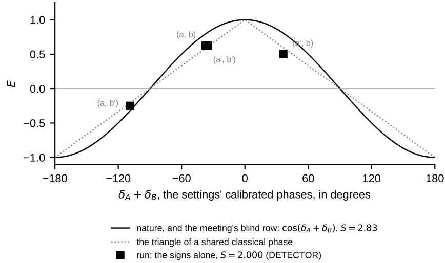
Fig. 7 Bell: the correlation E at the four settings against the sum of the settings' calibrated phases. The run by the signs alone on both sides, every quantum credited (the marks, DETECTOR), follows the triangle of a shared classical phase and sums to S = 2.000 ; the cosine is nature's E = \cos(\delta_A + \delta_B) and the meeting's blind row, S = 2.83 , for the run to come. Drawn from the rows of the law's document; no run of this paper's.
