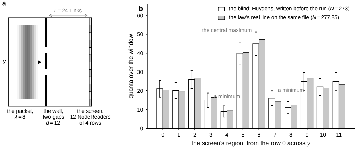
Fig. 6 The two slits, the one computed file (Sections 9.1 and 9.2; COMPUTED, CLICKS). (a) Universe24 as its file declares it. The flat GameBoard has 45 \times 48 Nodes. The packet of light, at the wavelength 8 Links, is laid over the columns 4 to 16 (the grey raised cosine) and moves along +x . The wall at the column 20 has two gaps of three rows, 12 Links apart. The screen at the column 44, 24 Links from the wall, is twelve declared NodeReaders of four rows each. (b) The screen's row per region over the window of the intervals 45 to 130. The Huygens blind, written before the run, is hollow ( N = 273 , with the draw's scatter \sqrt{Np(1-p)} per region). Beside it, in grey, is the law's real line stepped on the same file, as recorded in two_slits_real_line.txt by the reader of the paper's script two_slits_real_line.py (its script does not import at the pinned commit, Section 3.7) ( N = 277.85 in the engine's labels, 278.0 in the physical ones). The run of the implementation gives N = 270 (Section 3.7; 278 at the lay before the fix of PR #1862). The numbers drawn are the blind file's and the script's; nothing is read from a run of the engine for the drawing.
