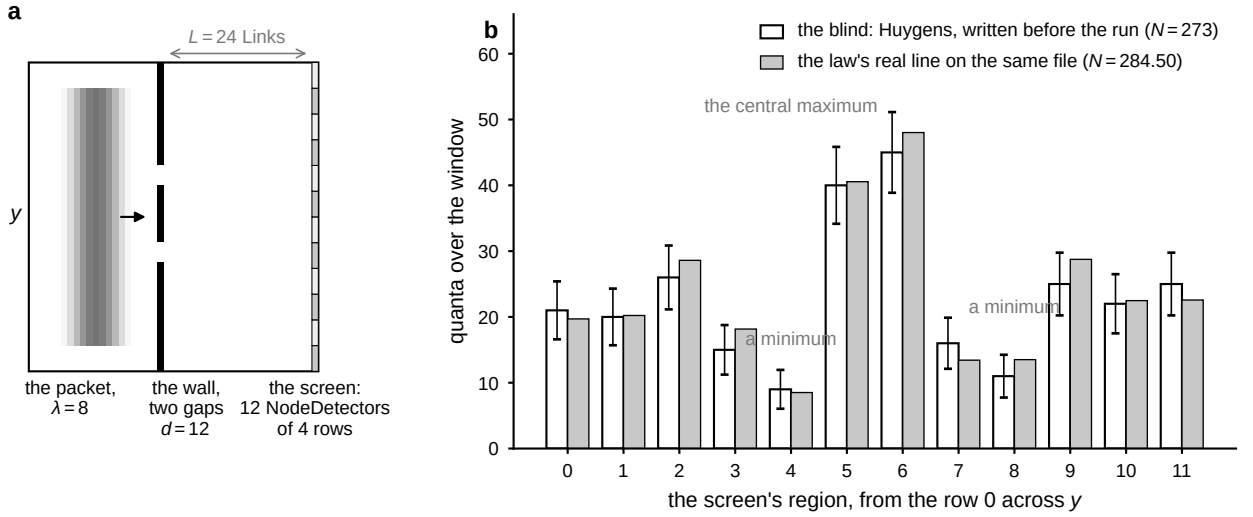
Fig. 6 The two slits, the one computed file (Sections 9.1 and 9.2; COMPUTED , CLICKS ; two.slits.rows.py ). (a) Universe24 as its file declares it. The flat lattice has 45 \times 48 Nodes. The packet of light, at the wavelength 8 Links, is laid over the columns 4 to 16 (the grey raised cosine) and moves along +x . The wall at the column 20 has two gaps of three rows, 12 Links apart. The screen at the column 44, 24 Links from the wall, is twelve declared NodeDetectors of four rows each. (b) The screen's row per region over the window of the intervals 45 to 130. The Huygens blind, written before the run, is hollow ( N = 273 , its bars summing to 275 by the per-Node rounding, with the draw's scatter \sqrt{NP(1-P)} per region). Beside it, in grey, is the law's real line stepped on the same file, as printed in two.slits.real.line.txt by the paper's script two.slits.real.line.py at the lay as that commit holds it, the band's exact level ( N = 284.50 in the engine's labels, 284.7 in the physical ones; 278.89 when the laid record's own integers, laid at the content 60's paces, are stepped by this line at the content 0's). The run of the implementation gives N = 285 at both seeds (Section 3.7). The numbers drawn are the blind file's and the script's; nothing is read from a run of the engine for the drawing
