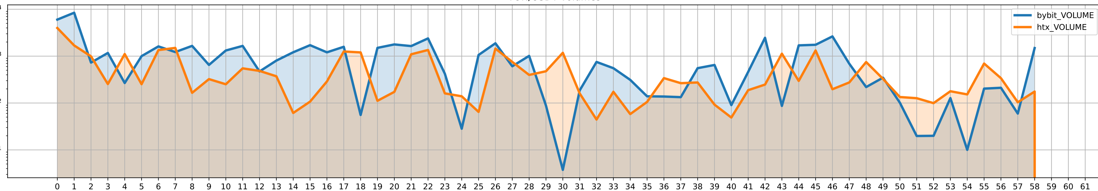
TON/USDT volumes
