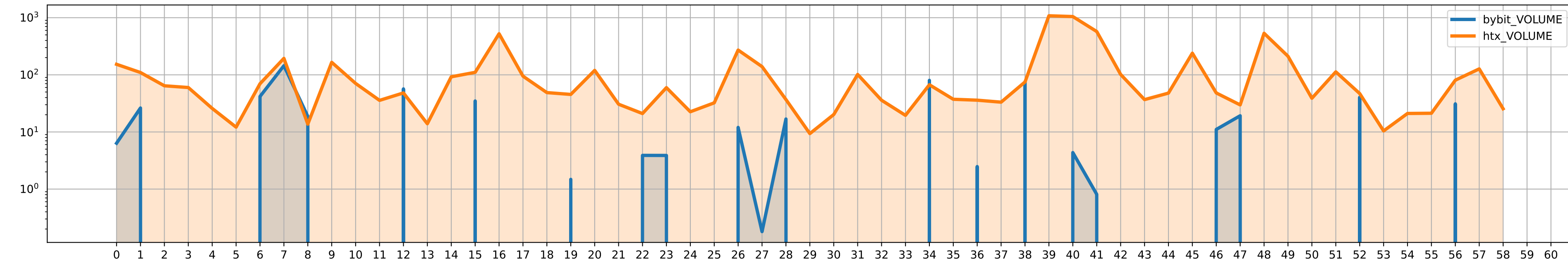
ETC/USDT volumes
