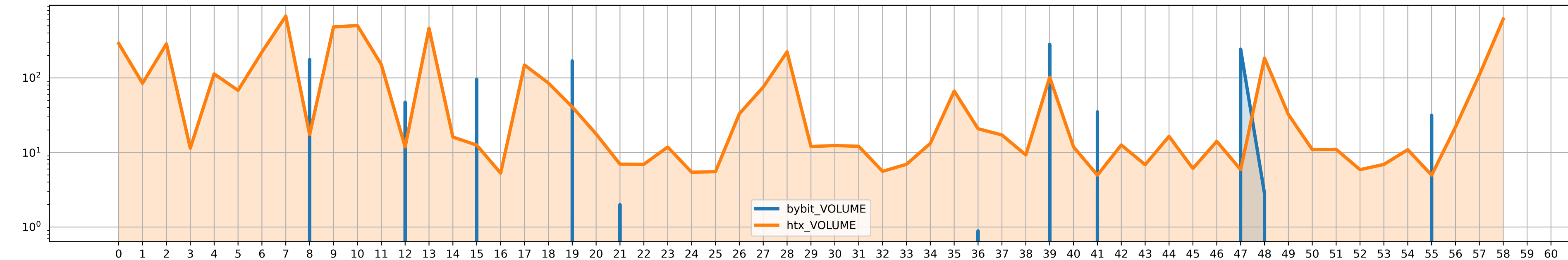
SSV/USDT volumes
