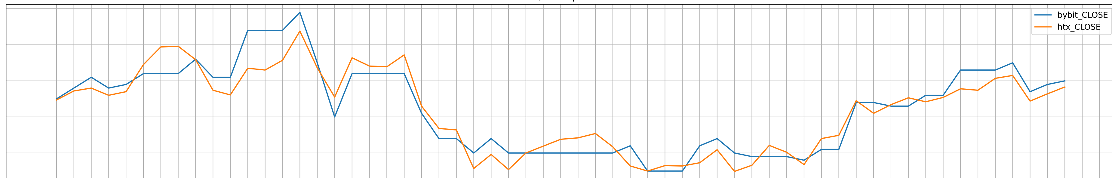
AXS/USDT % diff
