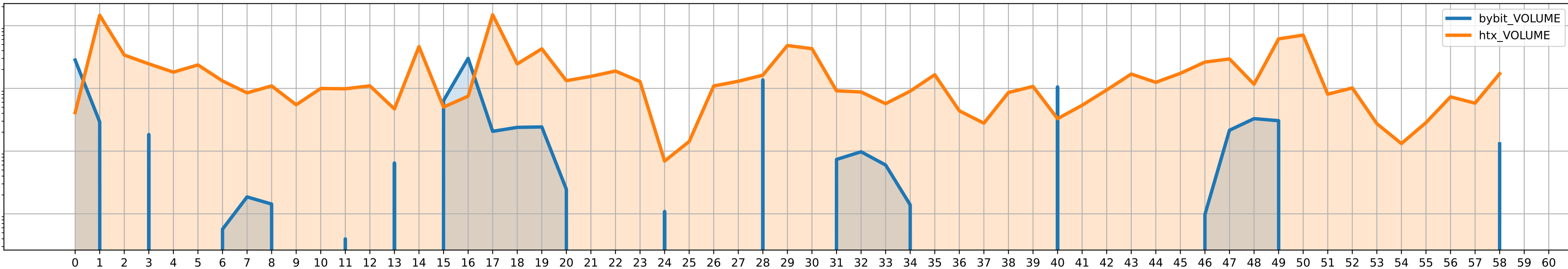
PENDLE/USDT volumes
