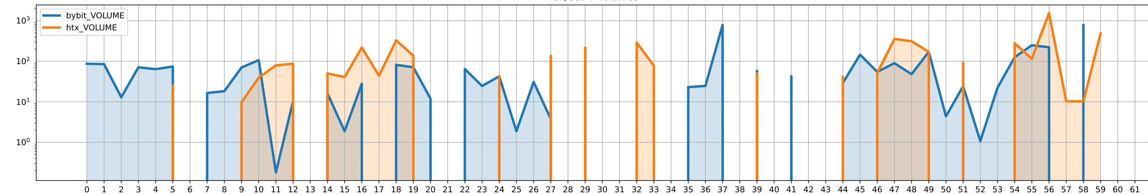
ICP/USDT volumes
