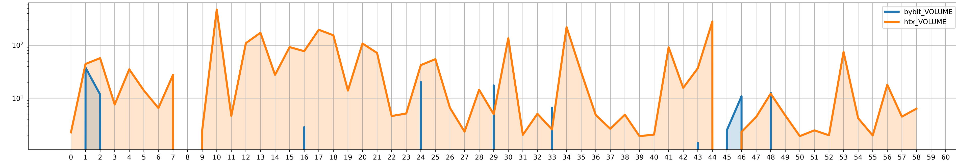
RPL/USDT volumes
