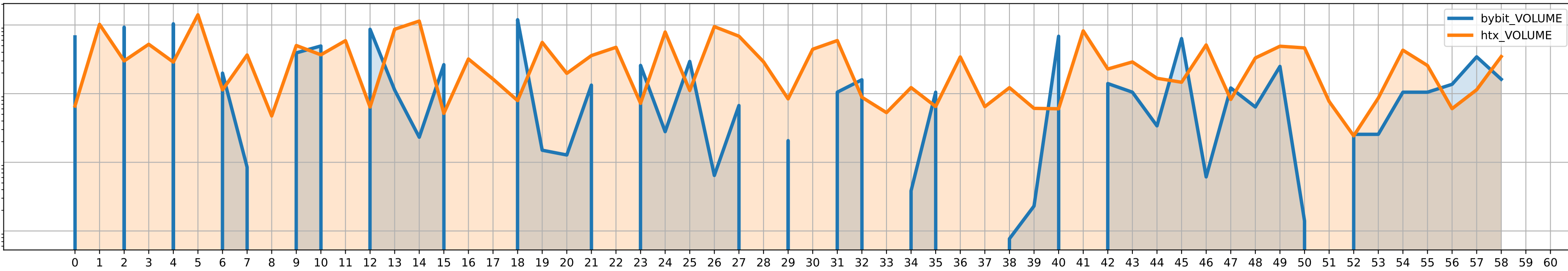
ATOM/USDT volumes
