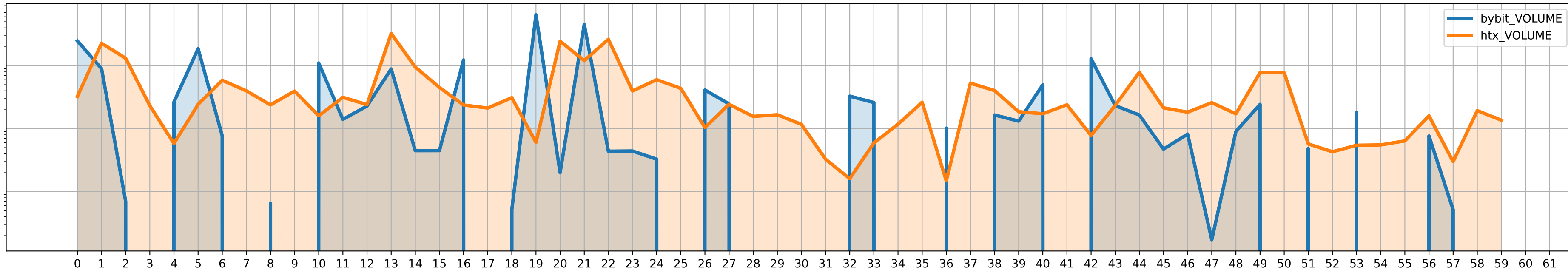
RENDER/USDT volumes
