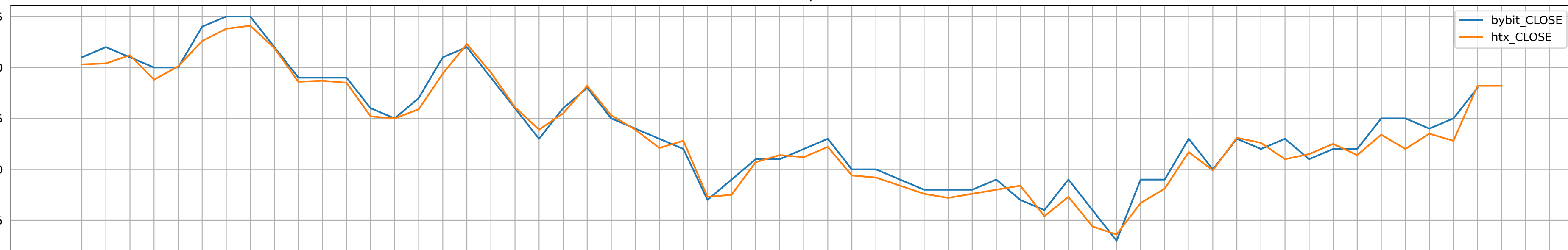
TON/USDT % diff
