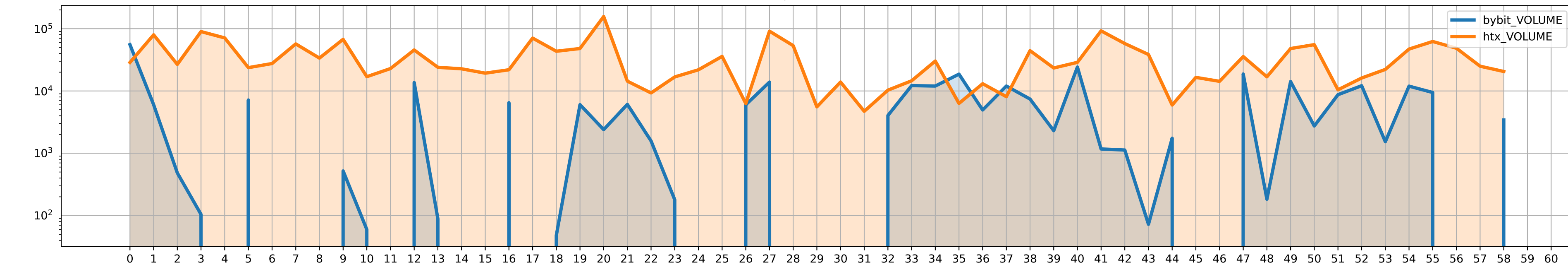
PNUT/USDT volumes
