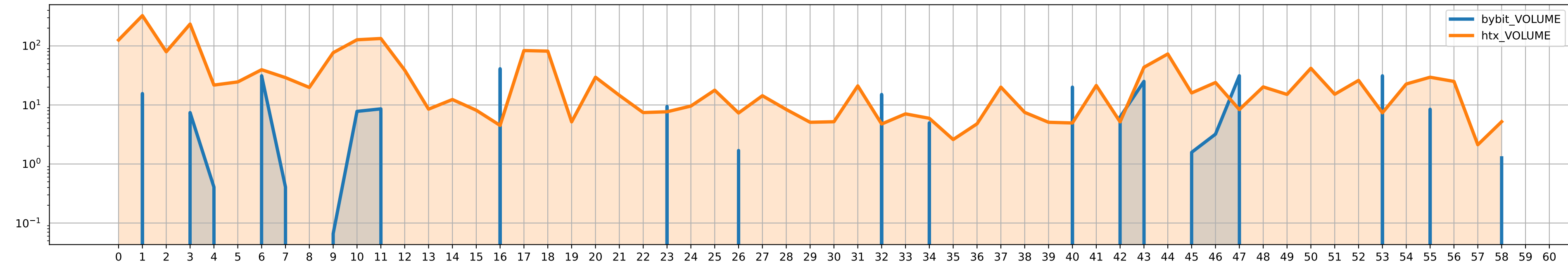
KSM/USDT volumes
