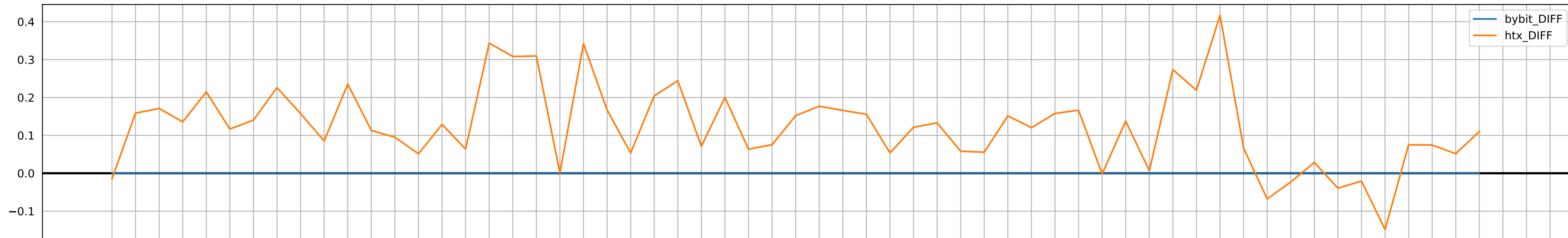
ENS/USDT % diff
