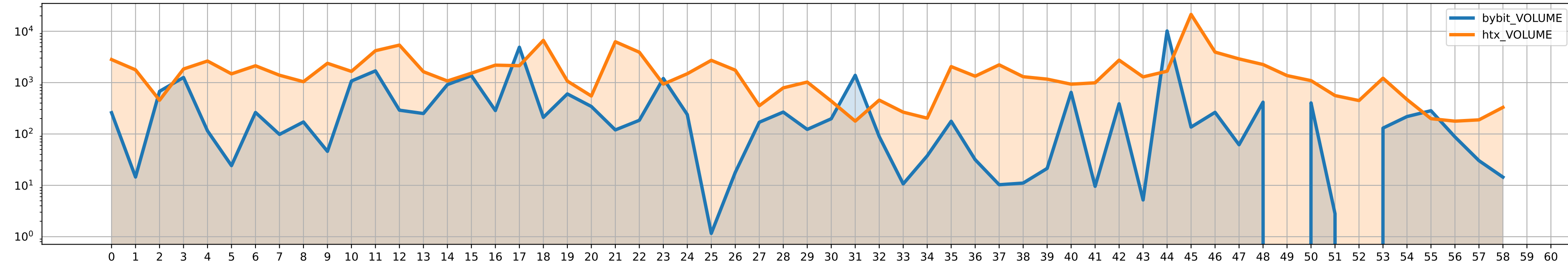
NEAR/USDT volumes
