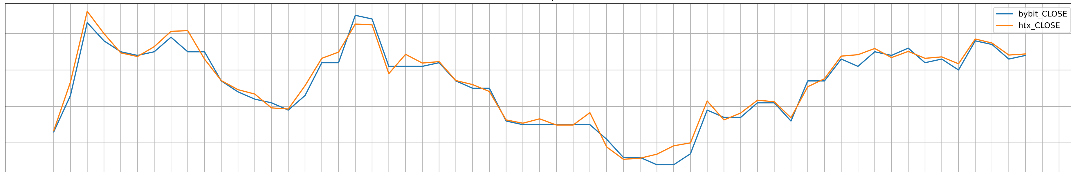
BCH/USDT % diff
