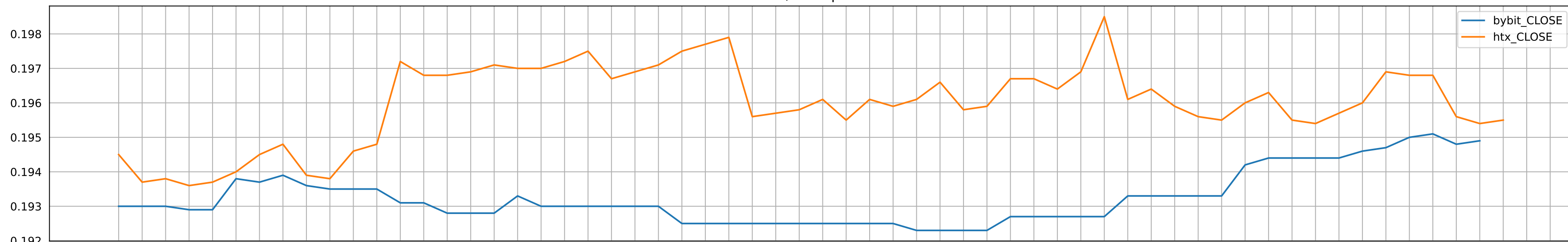
LUNA/USDT % diff
