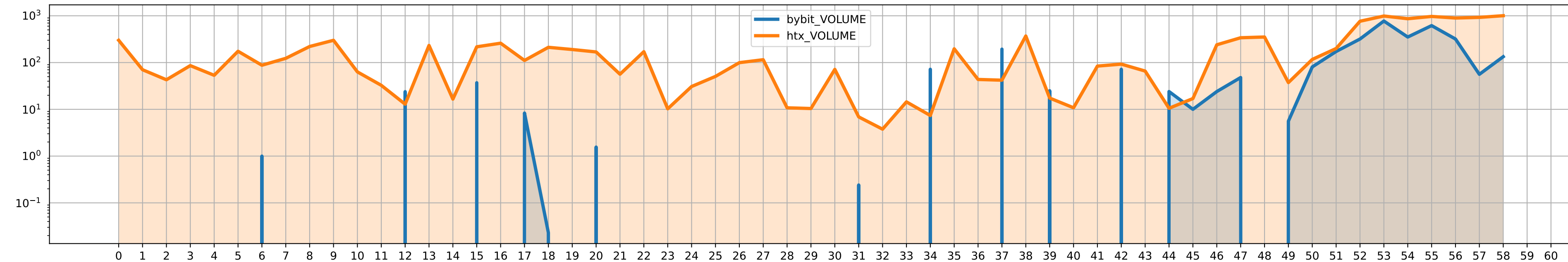
COMP/USDT volumes
