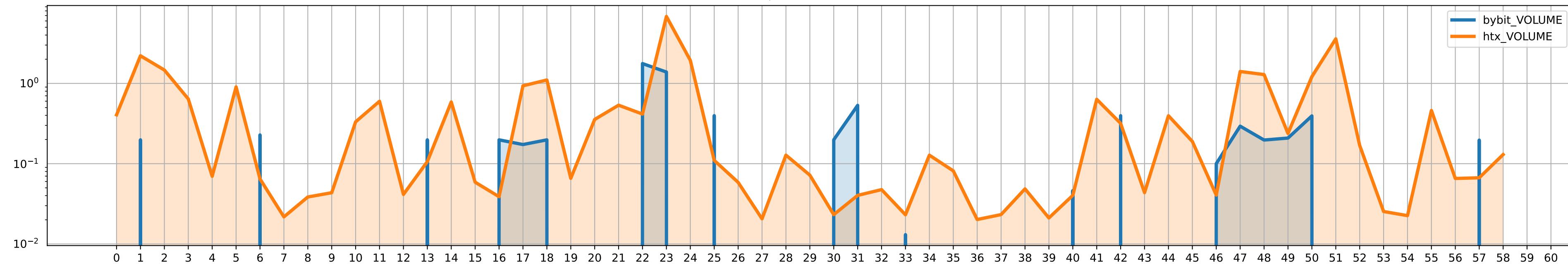
YFI/USDT volumes
