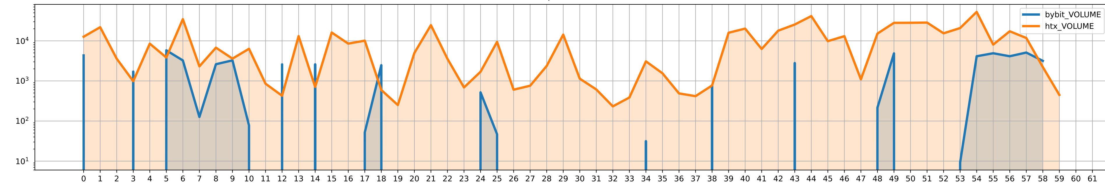
LUNA/USDT volumes
