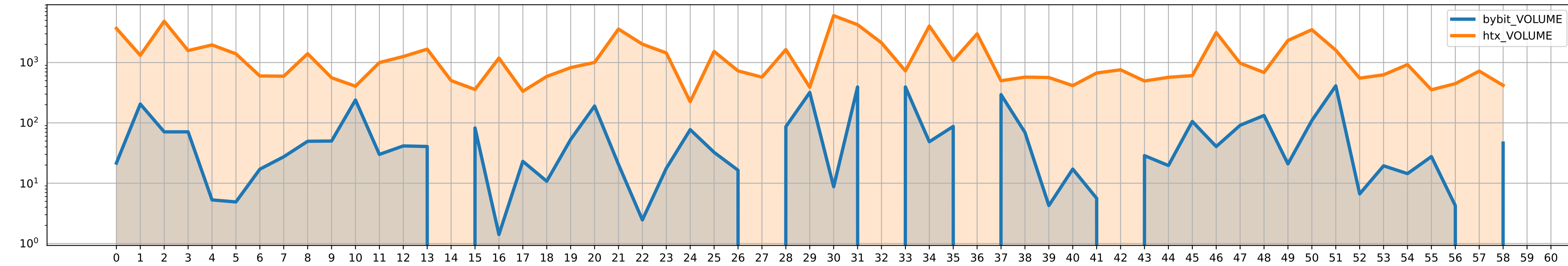
BERA/USDT volumes
