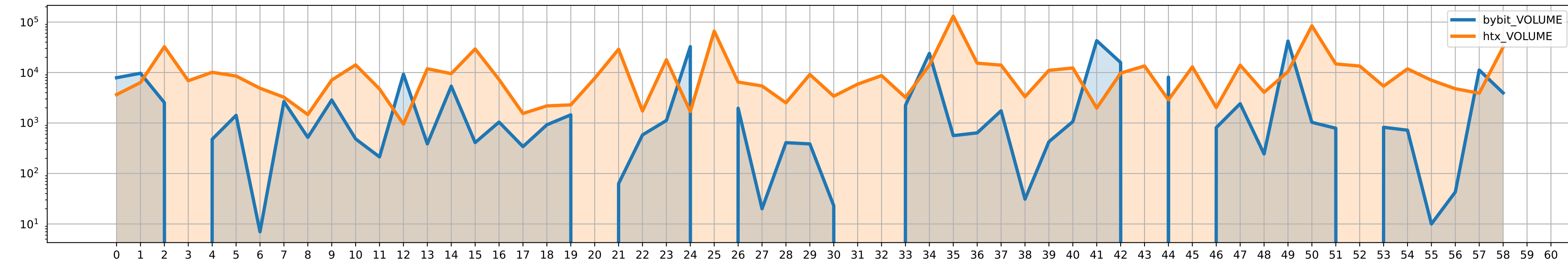
MOVE/USDT volumes
