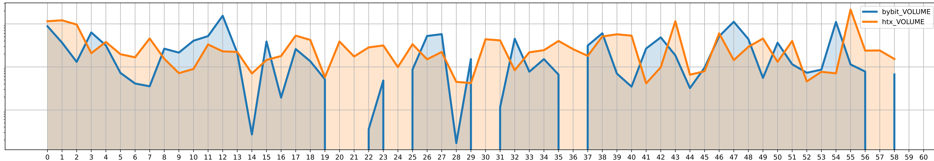
UNI/USDT volumes
