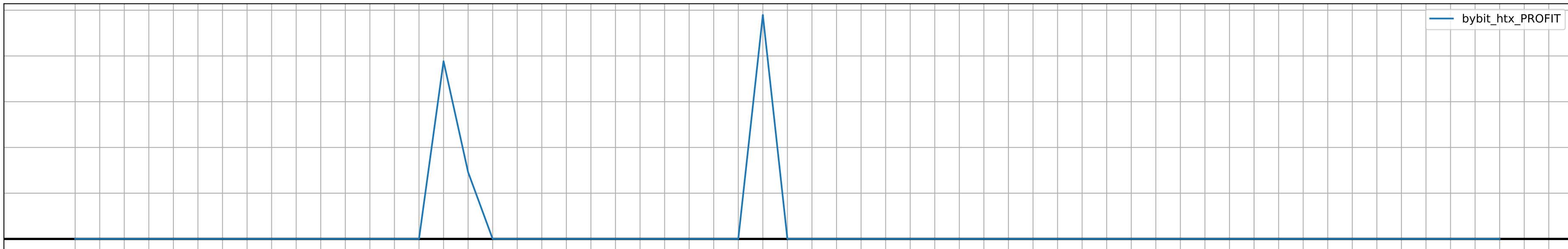
PENDLE/USDT volumes
