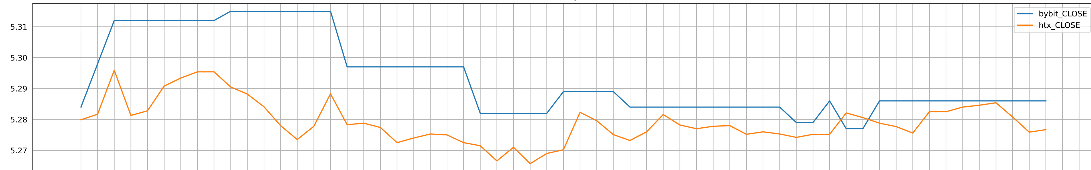
RPL/USDT % diff
