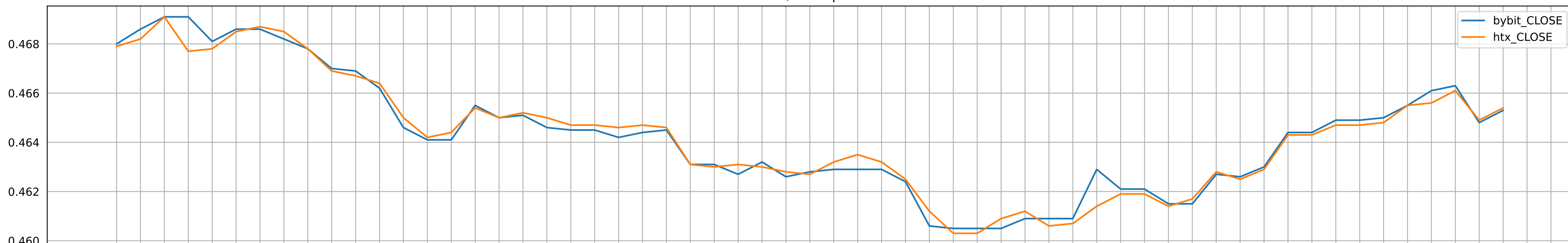
MOVE/USDT % diff
