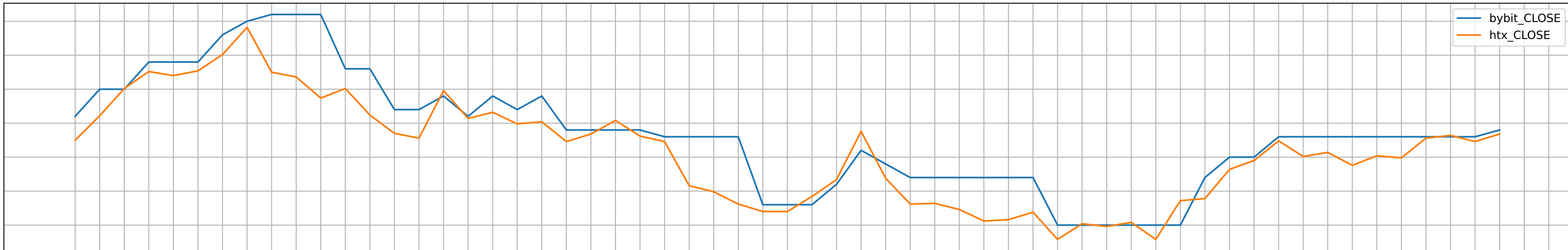
PENDLE/USDT % diff
