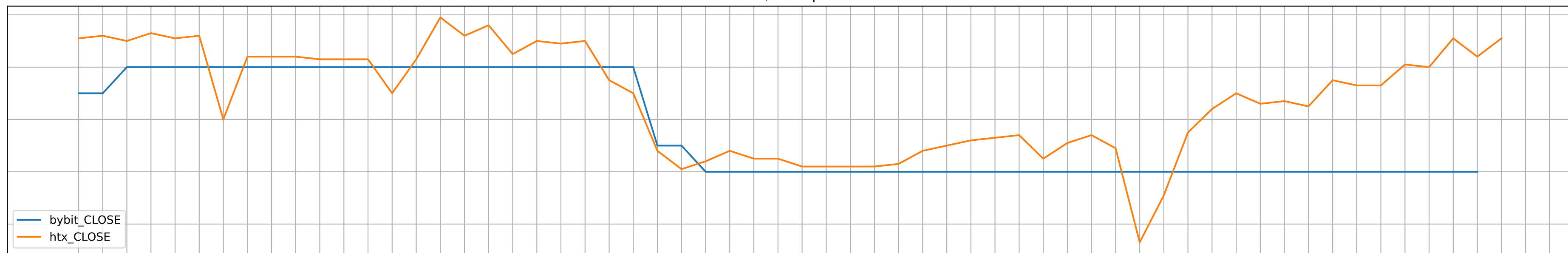
MASK/USDT % diff
