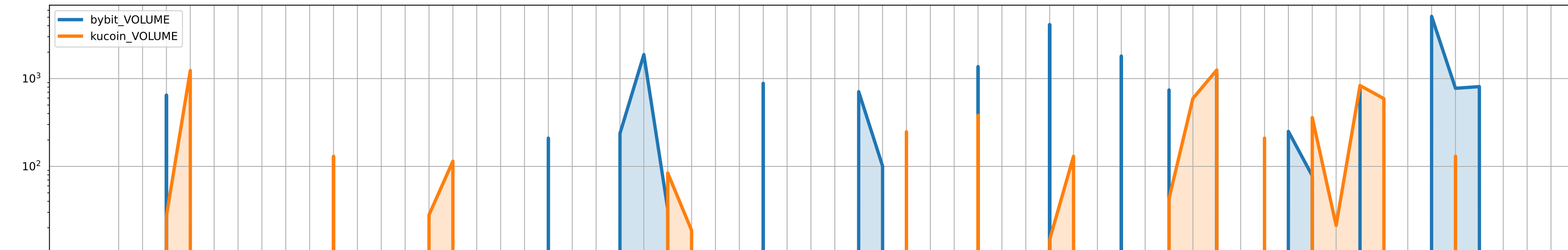
FLOW/USDT VOLUMES
