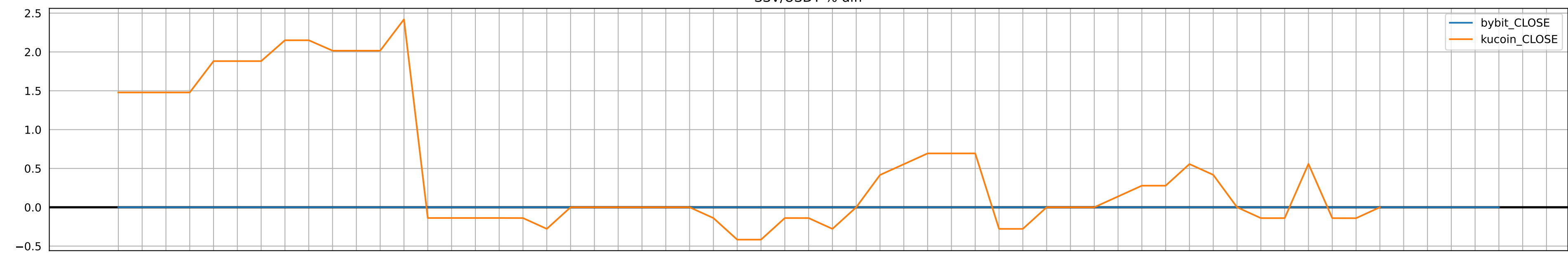
SSV/USDT % diff
