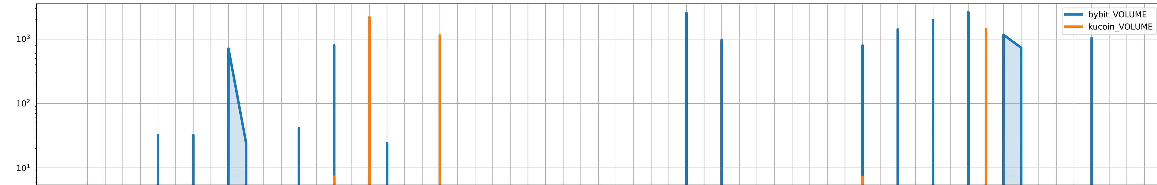
DYM/USDT VOLUMES
