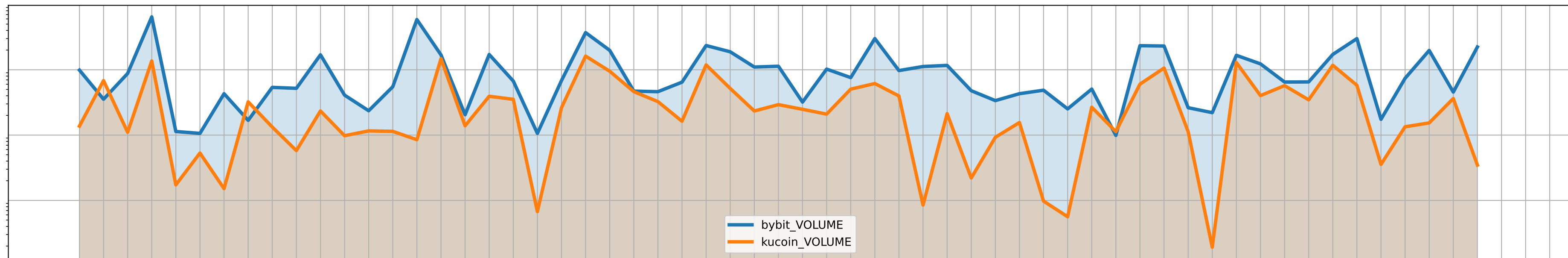
BNB/USDT VOLUMES
