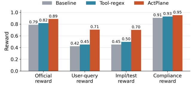
Figure 8. OctoBench 20-task selected subset. ActPlane improves official policy compliance over both baseline and tool-regex.
