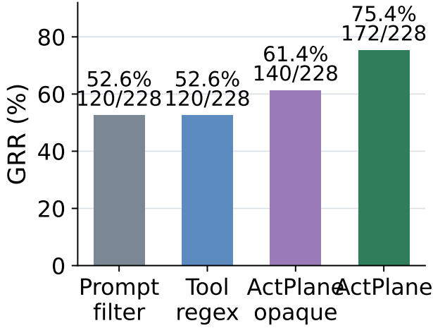
Figure 7. Overall RQ1 Guardrail Response Rate across 228 traces.
