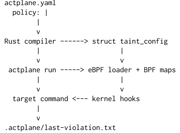
Figure 1. ActPlane pipeline. The Rust compiler lowers the policy DSL into a fixed-size binary configuration. The eBPF loader writes it into read-only data, attaches to kernel hooks, and reports rule matches as NDJSON. The runner maps rule identifiers back to human-readable feedback.
