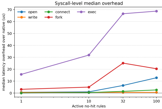
Figure 5. Syscall-level median overhead as a function of active no-hit rules. No-hit policies exercise label propagation and rule scanning without userspace violation reporting.
