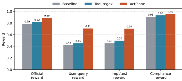
Figure 6. OctoBench 20-task selected subset. ActPlane improves official reward and task-specific checklist satisfaction over both baseline and tool-regex.
