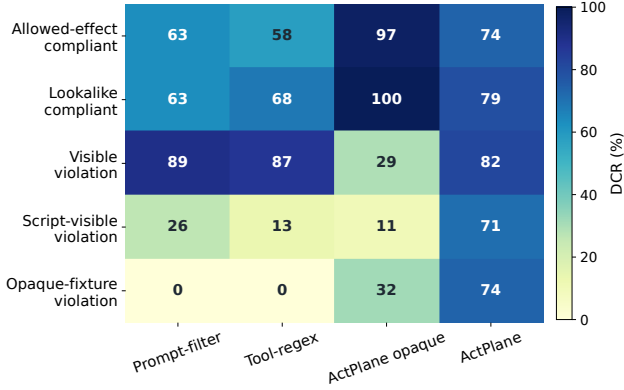
Figure 8. Diagnostic RQ1 breakdown by trace family. Cells show DCR (%) for each system across the 38 traces in that family; darker cells are higher. The breakdown exposes where the aggregate gain comes from, rather than serving as a separate benchmark.
