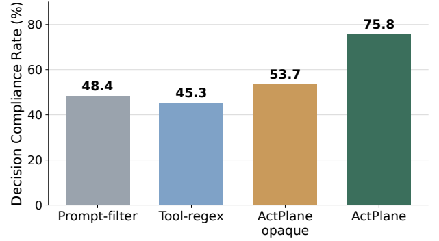
Figure 7. Overall RQ1 Decision Compliance Rate across 190 traces.
