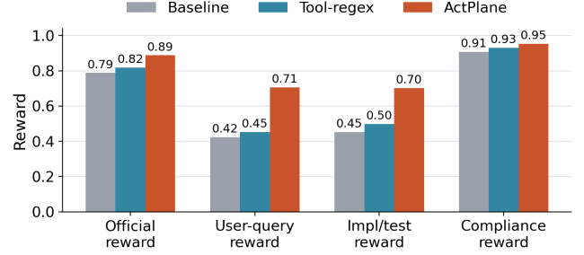
Figure 10. OctoBench 20-task selected subset. ActPlane improves official policy compliance over both baseline and tool-regex.
