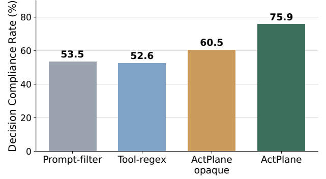
Figure 7. Overall RQ1 Decision Compliance Rate across 228 traces.
