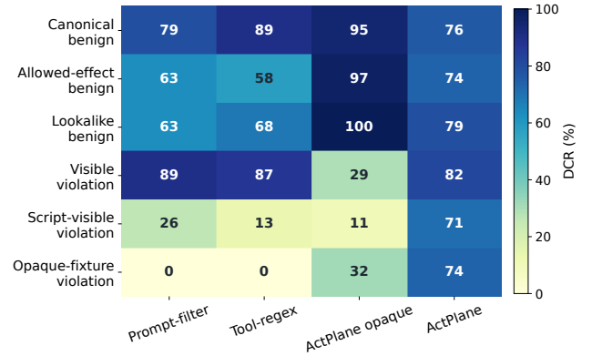
Figure 8. Diagnostic RQ1 breakdown by trace family. Cells show DCR (%) for each system across the 38 traces in that family; darker cells are higher. The breakdown exposes where the aggregate gain comes from, rather than serving as a separate benchmark.
