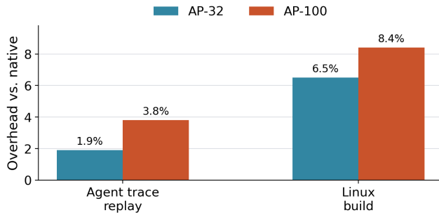
Figure 7. End-to-end overhead on deterministic workloads, normalized to native execution. At 32 active no-hit rules, ActPlane adds 1.9% on agent-trace replay and 6.5% on a Linux build; at 100 rules, overhead remains below 8.4%.
