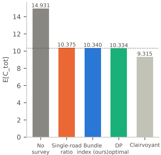
(a) Expected total cost (dotted: J(s_0) )
