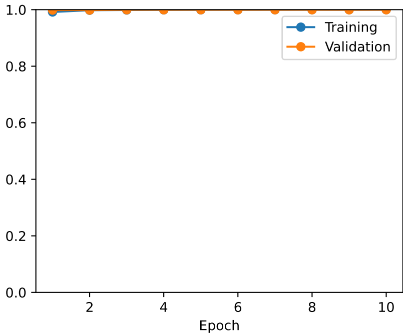
Accuracy
