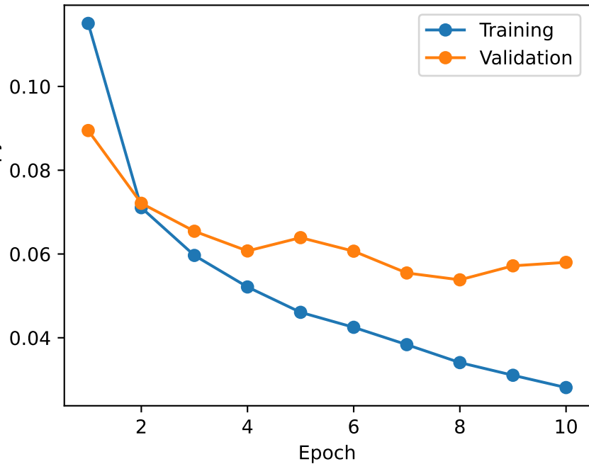
Cross-entropy
