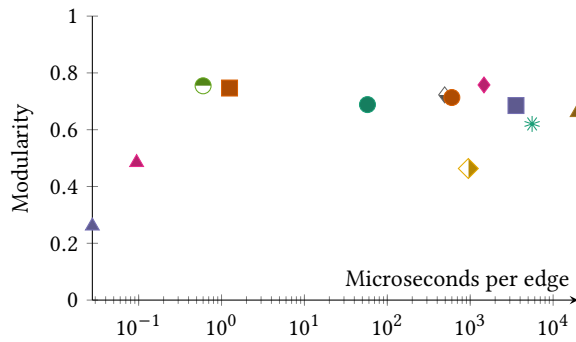
Figure 3: Ratio between time per edge and quality, using the geometric mean for both measures. This plot shares legend with Figure 1. Parallel algorithms have two connected points, showing parallel and sequential versions.
