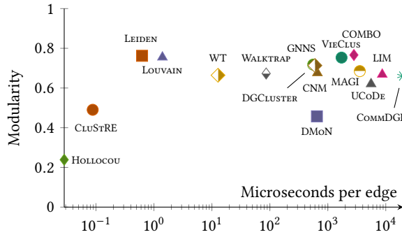
Figure 4: Scatter plot showing the ratio between running time and solution quality, using the geometric mean for both measures. To normalize the running time per graph, we divide it by the number of edges, yielding a time-per-edge measure.
