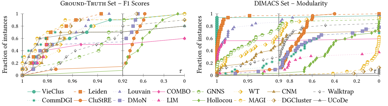
Figure 2: Performance profiles for our first two datasets. We use F1 scores for the GROUND-TRUTH set and modularity for the DIMACS instances. For clarity, we split the x-axis to highlight the differences between the best algorithms near one.
