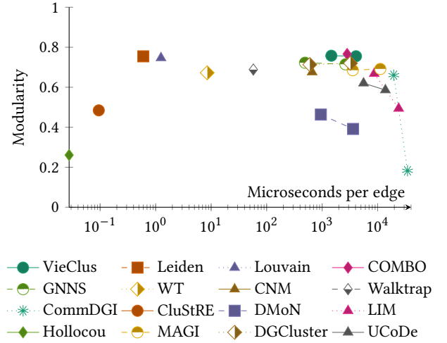
Figure 3: Ratio between time per edge and quality, using the geometric mean for both measures. Parallel algorithms have two connected points, showing parallel and sequential versions. For all the tested algorithms, the parallel versions had lower running times than the sequential versions, so the leftmost mark is always the parallel version.
