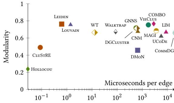
Figure 4: Scatter plot showing the ratio between running time and solution quality, using the geometric mean for both measures. To normalize the running time per graph, we divide it by the number of edges, yielding a time-per-edge measure.
