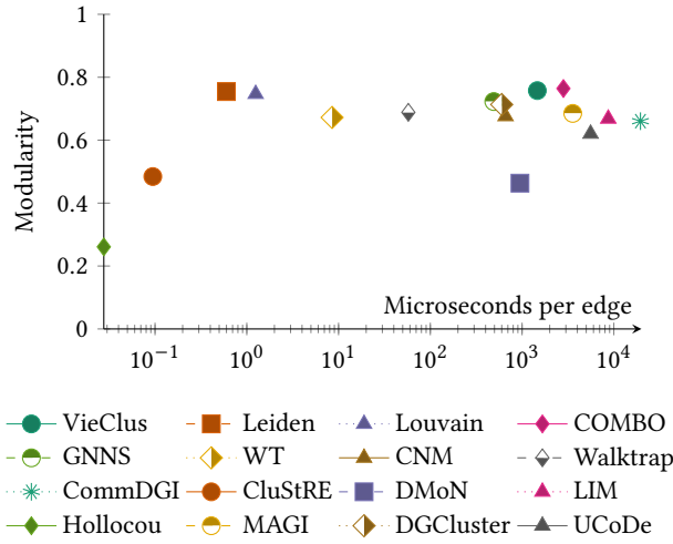
Figure 4: Scatter plot showing the ratio between running time and solution quality, using the geometric mean for both measures. To normalize the running time for each graph, we divide it by the number of edges, yielding a time-per-edge measure.
