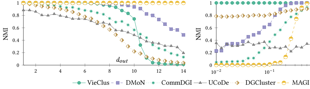
Figure 3: NMI scores on graphs generated with the ADC-SBM graph generator. All graphs have n = 1\,000 vertices, k = 4 clusters, d = 20 average degree, and \sigma = 1 intra-cluster center variance. The left plot varies d_{out} while keeping \sigma_c = 3 , and the right plot varies \sigma_c while keeping d_{out} = 2 .
