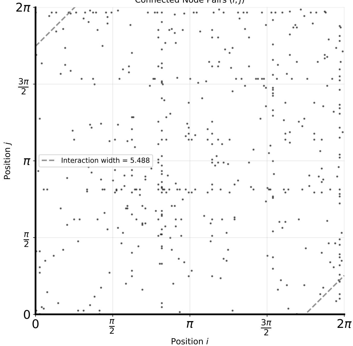
Connected Node Pairs (i, j)
