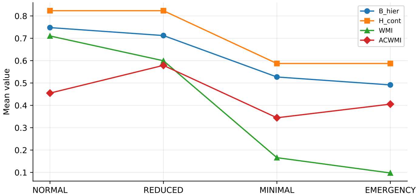
Fig. 8. Degradation levels vs breadth/honesty/world-model scores
