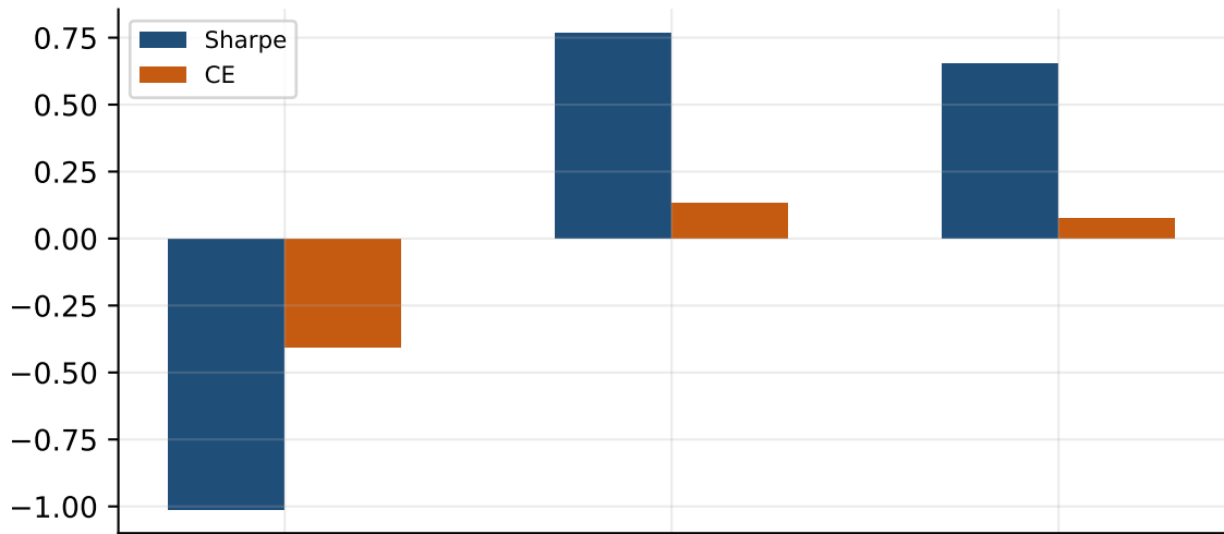
Fig. 6. Thin vs thick-ungated vs thick-gated worlds (OOS)
