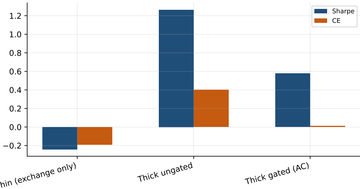
Fig. 6. Thin vs thick-ungated vs thick-gated worlds (OOS)
