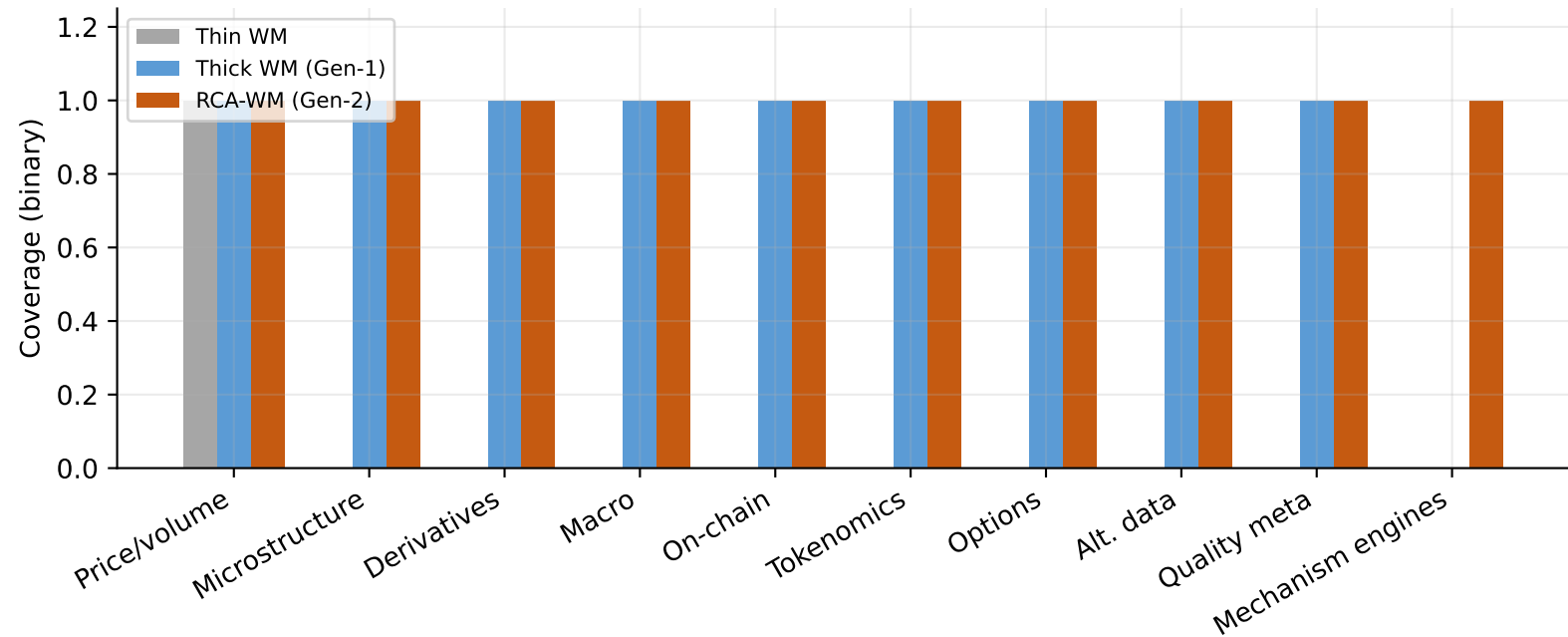
Fig. 2. Evidence coverage: thin vs thick vs RCA-WM
