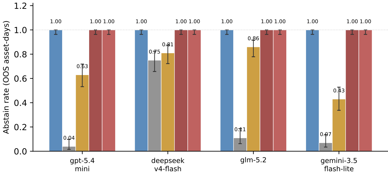
Live five-arm thin abstention (Wilson 95% CIs, n = 100 ; full-schema stress)
