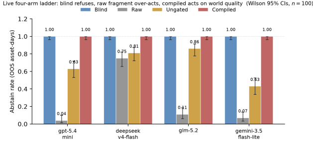
Figure 3: Live four-arm interface ladder (same 100 days; Wilson 95% CIs). Blind refuses; Raw over-trades; Ungated is vendor-dependent; Compiled enforces the typed refuse contract.
