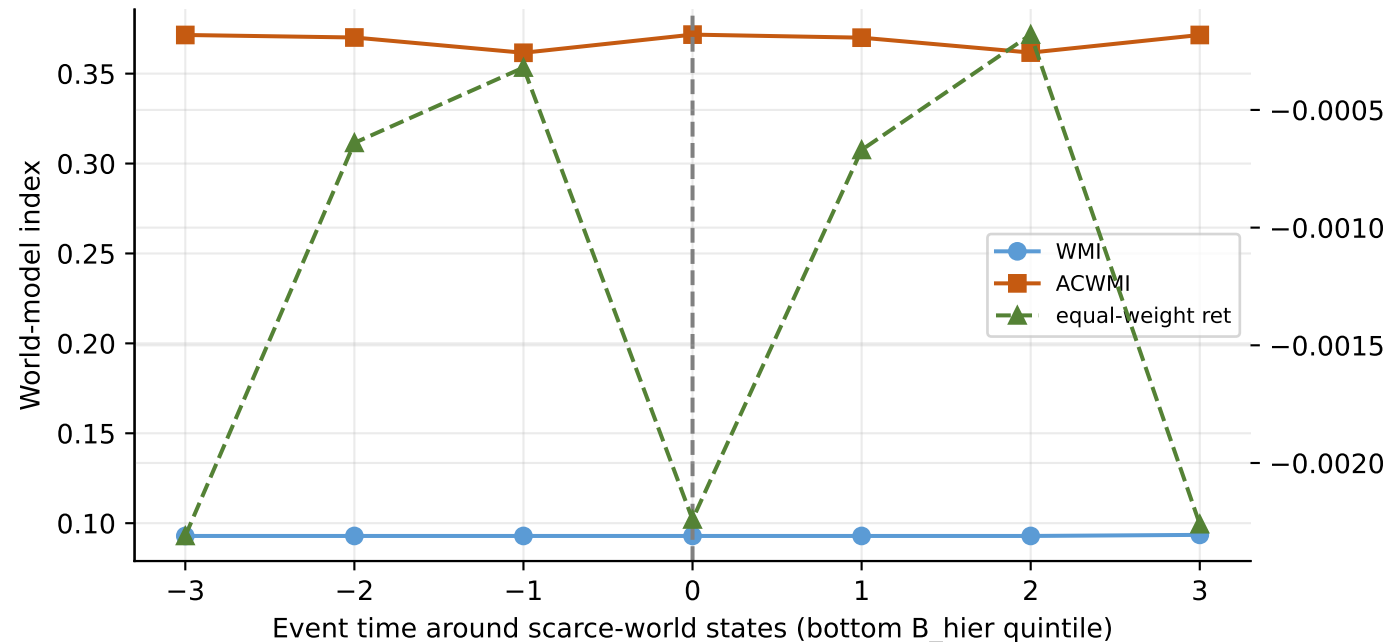
Fig. 5. Event study: real PIT scarce-world states
