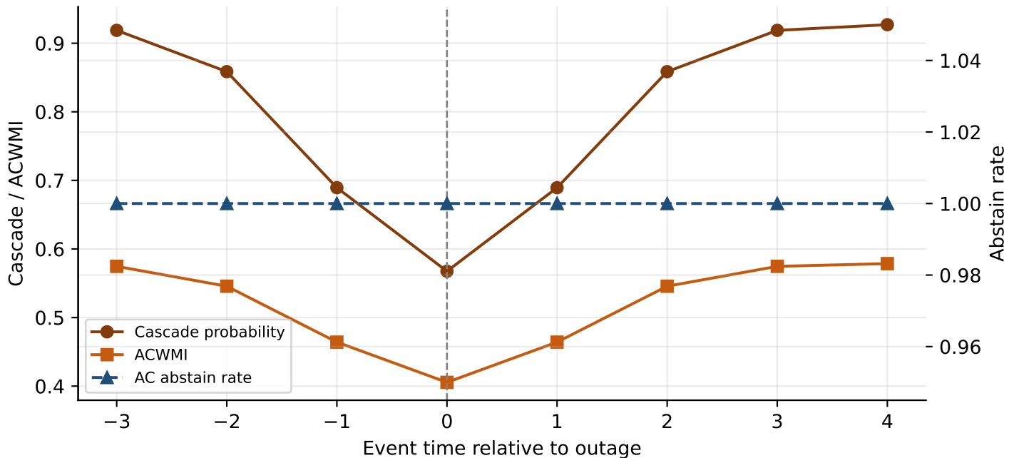
Fig. 6. Outage event profile in crisis regimes (project engines)
